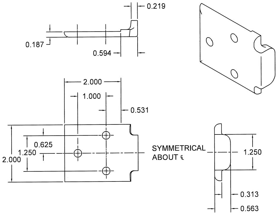
⑦ WINDLOCK DETAIL CAST MALLEABLE IRON ASTM A47, GRADE 32510, OR DUCTILE IRON PER ASTM A536 GRADE 65-45-12, GALVANIZED IN ACCORDANCE WITH ASTM A123, GRADE 85 ZINC-COATING 1/2 SCALE
