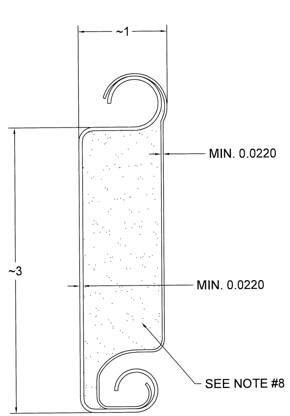
③ SLAT DETAIL TYPICAL SECTION
