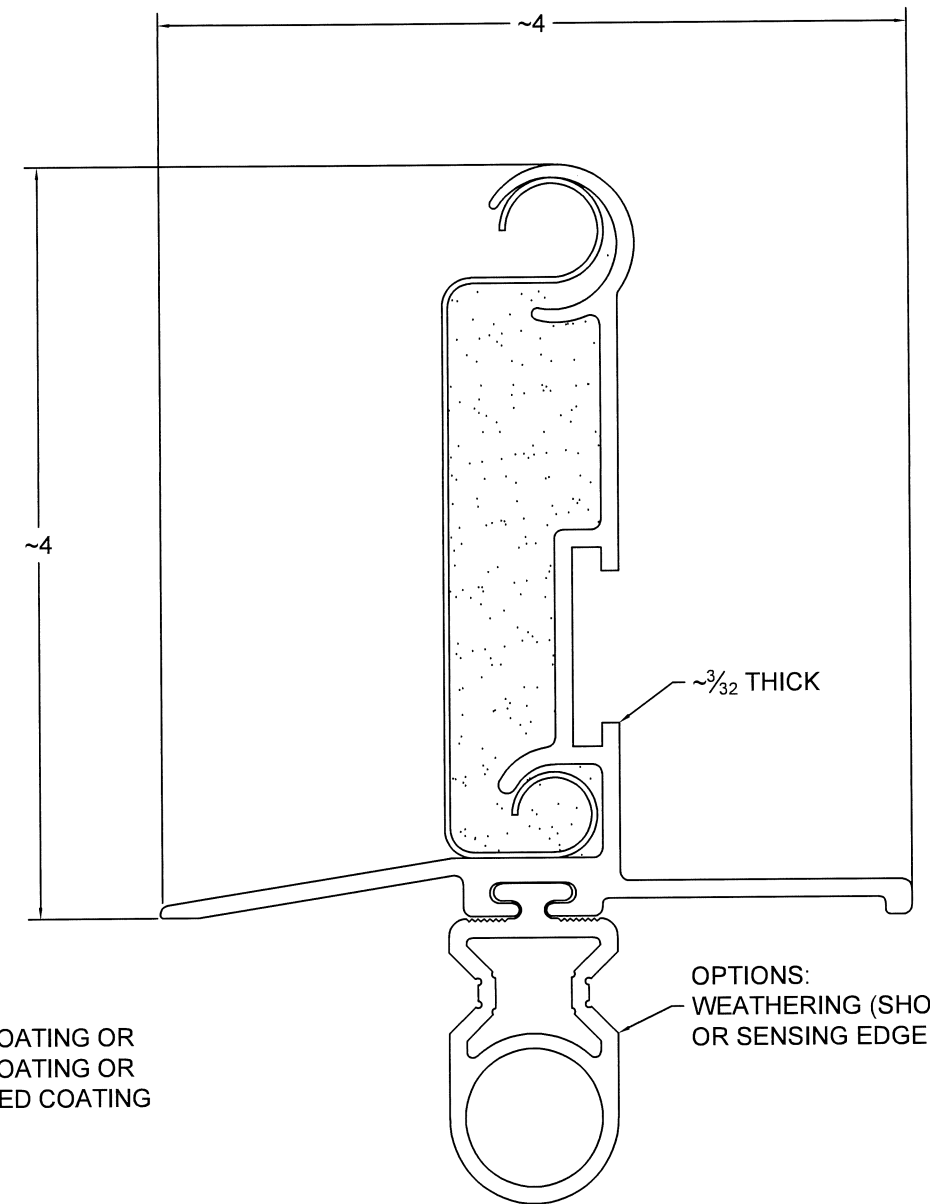
④ BOTTOM BAR DETAIL TYPICAL SECTION FULL SCALE 6063-T5 EXTRUDED ALUMINUM
