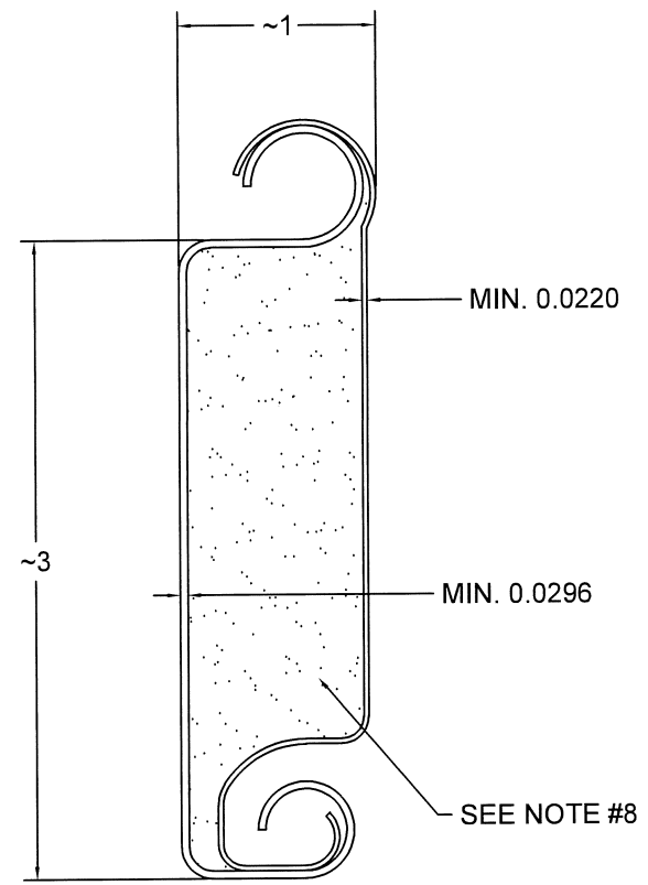
③ TYPICAL SECTION
