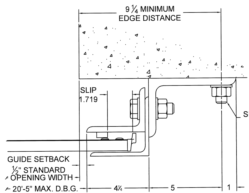
⑨ GUIDE ASSEMBLY CONCRETE STRUCTURE (Z-GUIDE)
