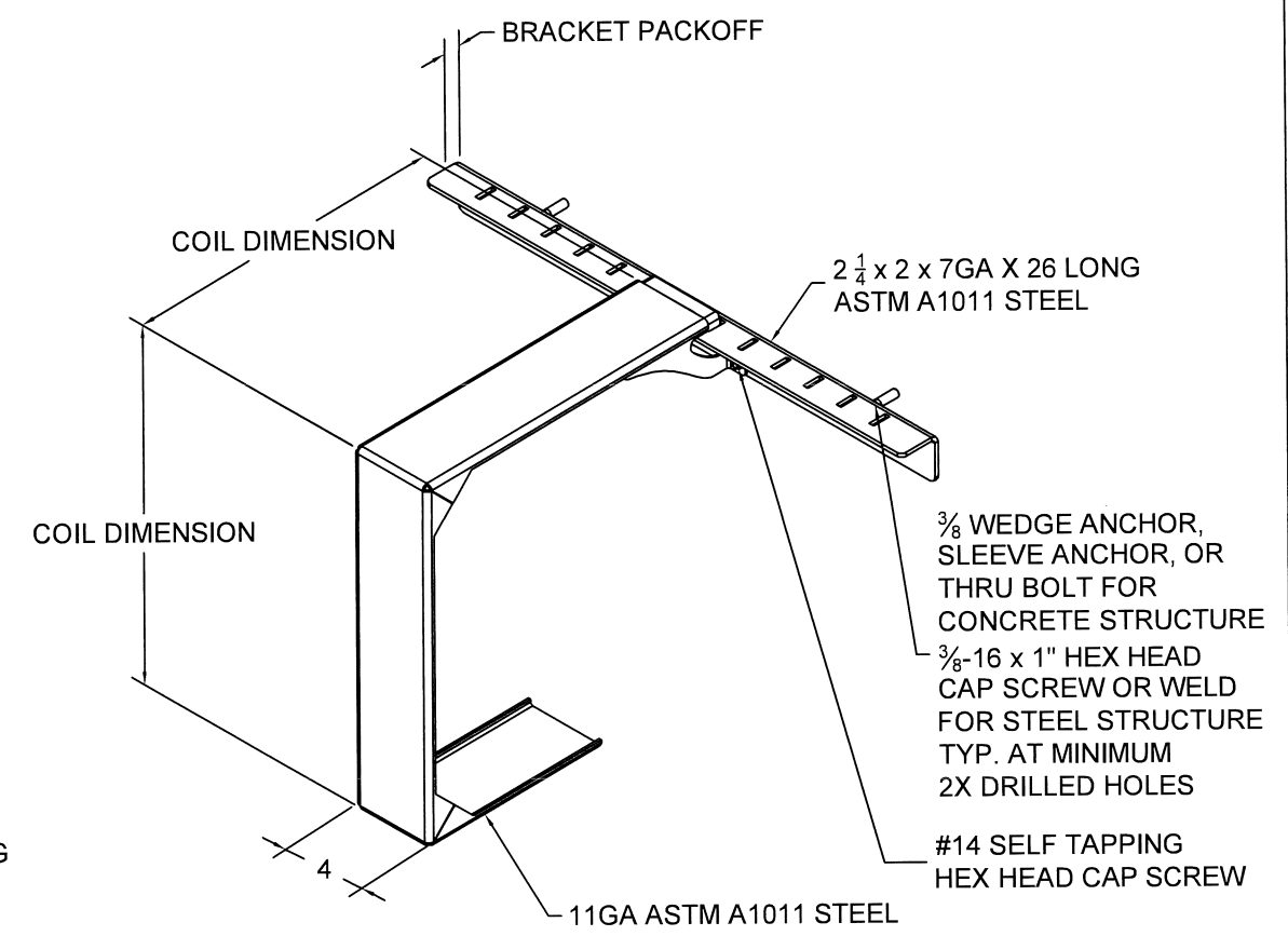
(18) MID-HOOD SUPPORT (WHEN REQUIRED) SQUARE STYLE DEPICTED, "D" SHAPE ALSO AVAILABLE SCALE: NTS
