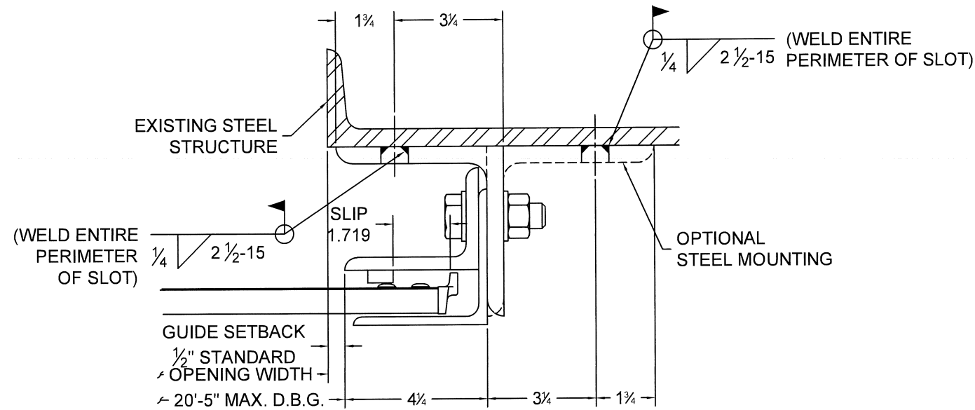
12 GUIDE ASSEMBLY STEEL STRUCTURE (Z-GUIDE OR E-GUIDE)
