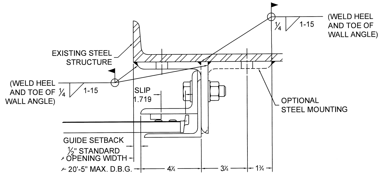
13 GUIDE ASSEMBLY STEEL STRUCTURE (Z-GUIDE OR E-GUIDE)
