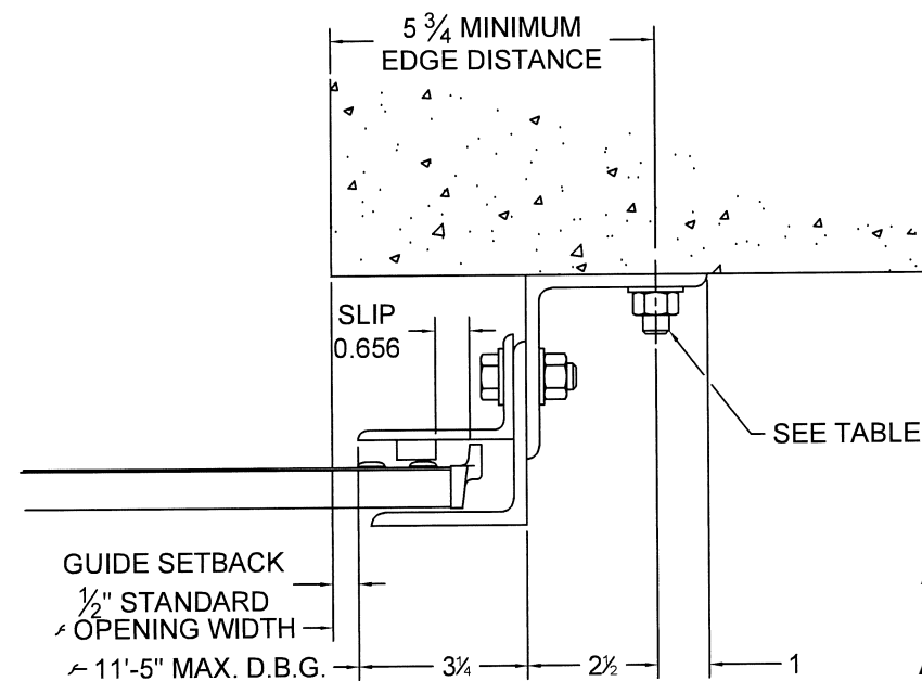
⑨ GUIDE ASSEMBLY CONCRETE STRUCTURE (Z-GUIDE)
