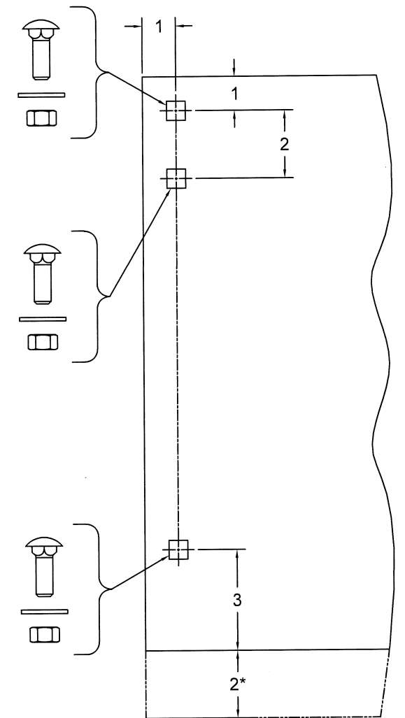
⑧ BRACKET MOUNTING DETAIL 0.172 MIN. THICKNESS
