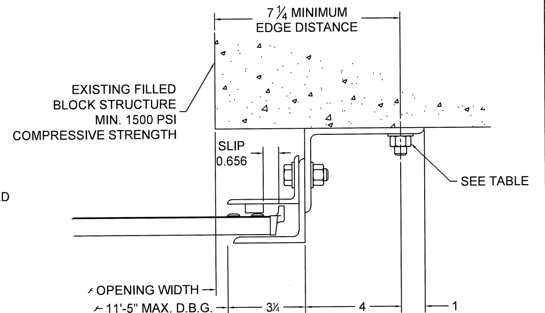
⑪ GUIDE ASSEMBLY FILLED BLOCK STRUCTURE (Z-GUIDE)
