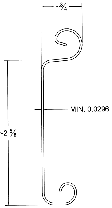
③ SLAT DETAIL TYPICAL SECTION
