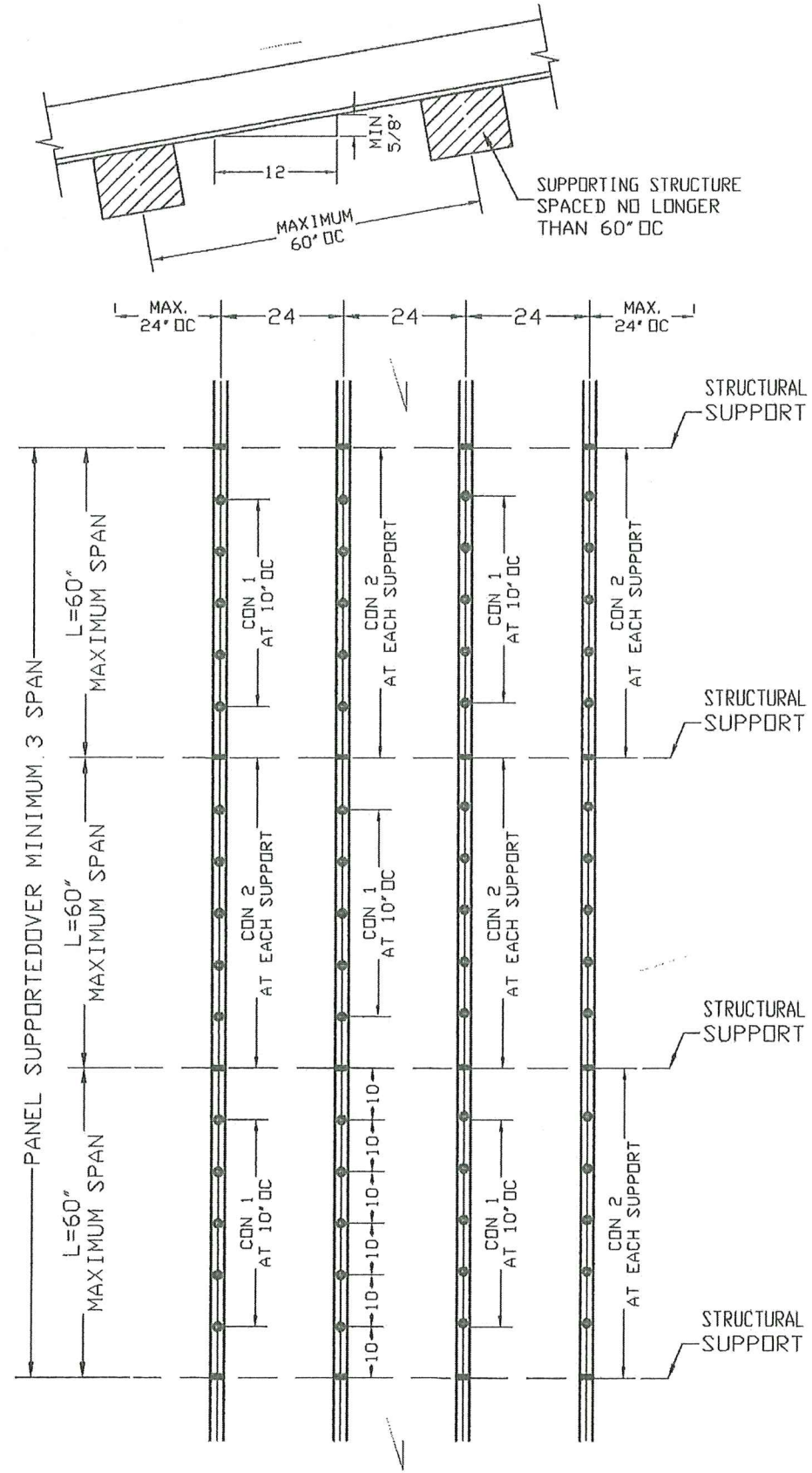
TYPICAL PANELS LAY-OUT AND ASSEMBLY AND ANCHORAGE TO STRUCTURAL SUPPORT
