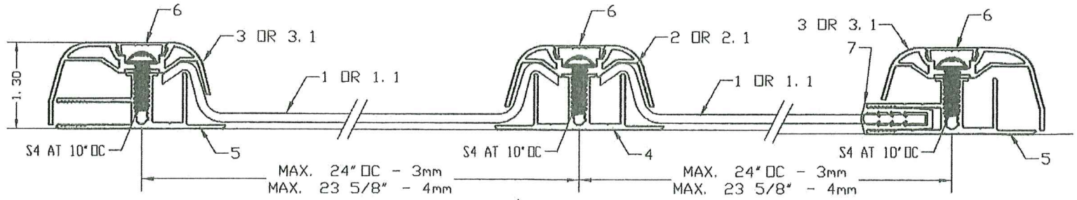
CON 1: CONNECTION IN BETWEEN SUPPORTS SPACED AT MAXIMUM 10' OC
