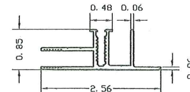
5- 3mm-4mm SIDE BASE #SAP 9014253
