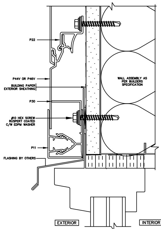
B 6 2-PC J TRIM WINDOW HEAD NOT-TO-SCALE | ELEVATION
