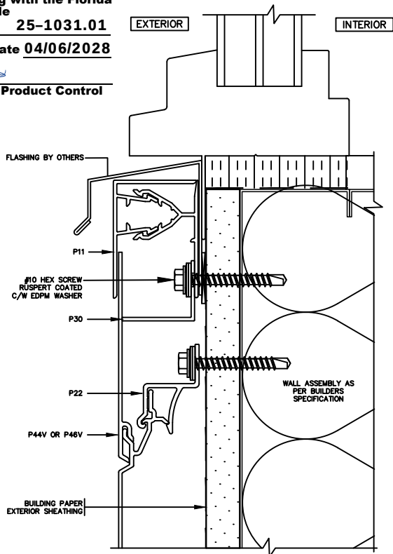
A 6 2-PC J TRIM WINDOW SILL NOT-TO-SCALE | ELEVATION
