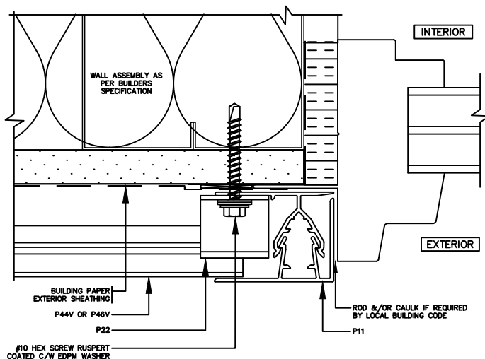
C 6 2-PC J TRIM WINDOW JAMB NOT-TO-SCALE | PLAN
