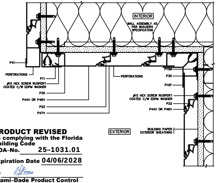
B 8 SOFFIT W/ INSIDE CORNER & 2-PIECE J TRIM NOT-TO-SCALE | ELEVATION
