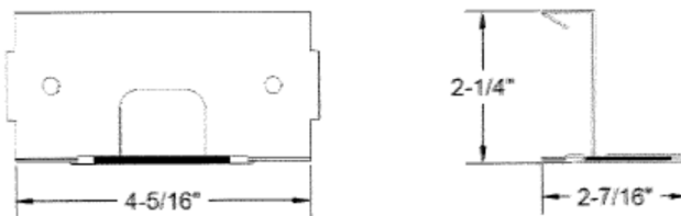
TWO-PIECE CLIP
