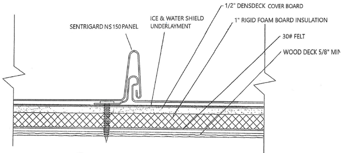
PANEL ASSEMBLY VIEW (WITHOUT STEEL STRAP)
