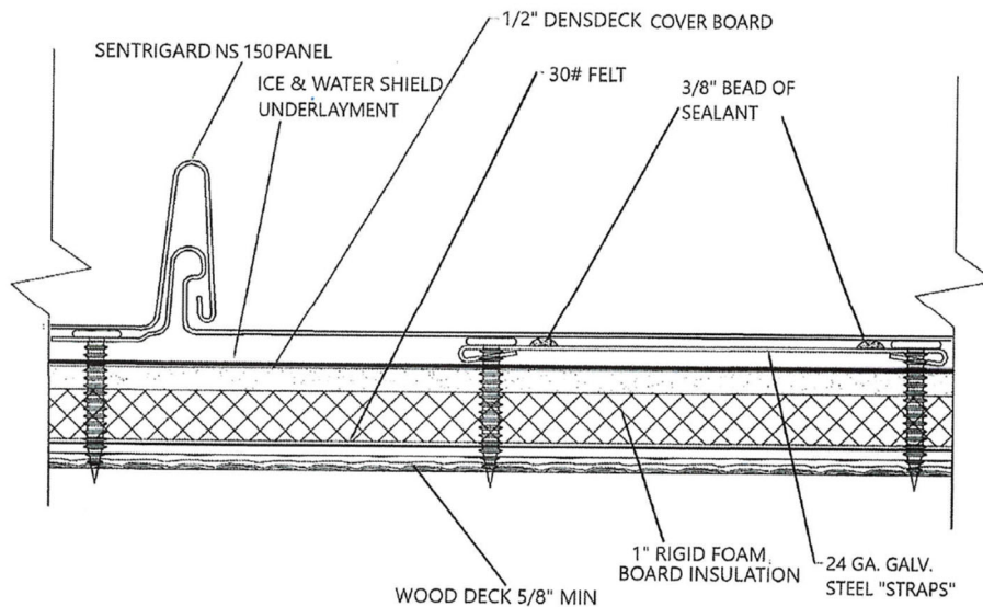
PANEL ASSEMBLY VIEW (WITH STEEL STRAP)
