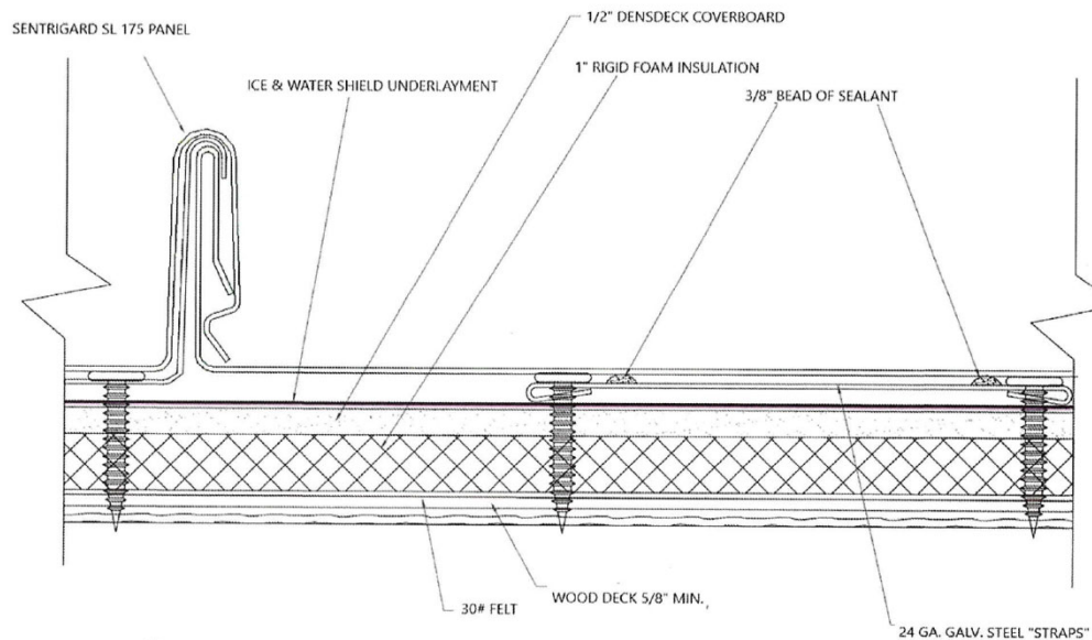
PANEL ASSEMBLY VIEW (WITH STEEL STRAP)
