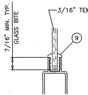
3/16 TEMP. GLAZING DETAIL
