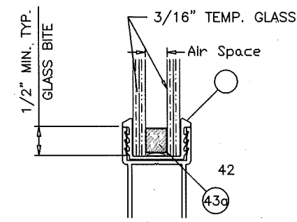
5/8 TEMP. INSULATED GLAZING DETAIL
