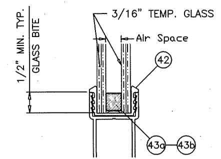
5/8 TEMP. INSULATED GLAZING DETAIL
