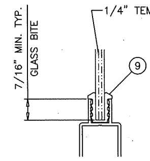
1/4 TEMP. GLAZING DETAIL
