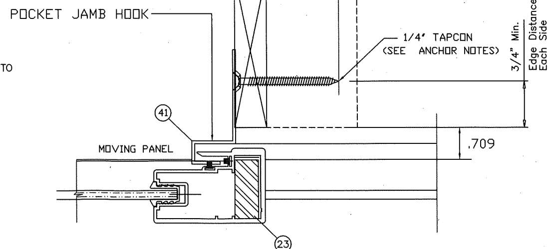
POCKET DOOR JAMB ANCHOR DETAIL
