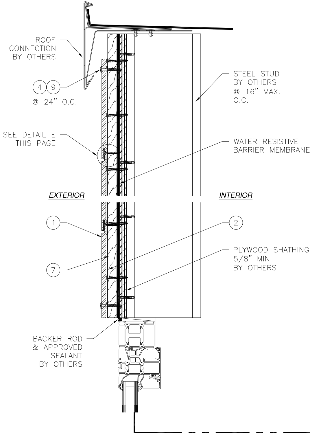
VERTICAL CROSS SECTION FLUSH SIDING INSTALLATION 5/8" MIN. PLYWOOD SHEATHING (METAL FRAME)
