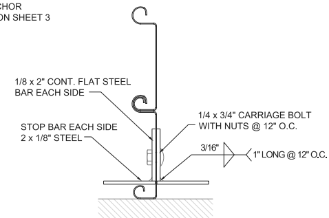
D BOTTOM BAR DETAIL
