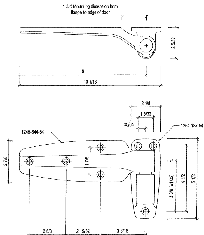
8 DOOR HINGE Model #1245 N.T.S.
