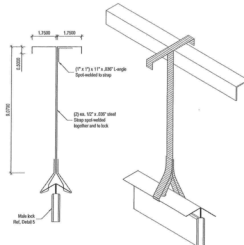
13 MALE LOCK W/ STRAP & ANGLE
