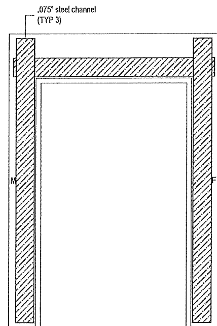
DOOR SECTION SHOWING EXTERIOR CHANNEL REINFORCEMENT
