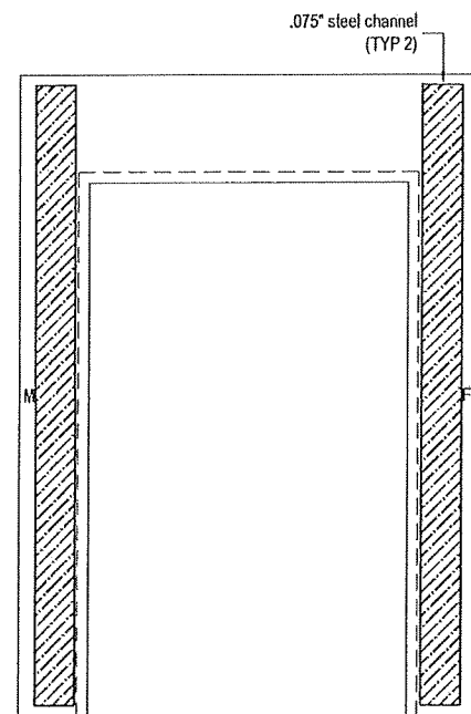
DOOR SECTION SHOWING INTERIOR CHANNEL REINFORCEMENT
