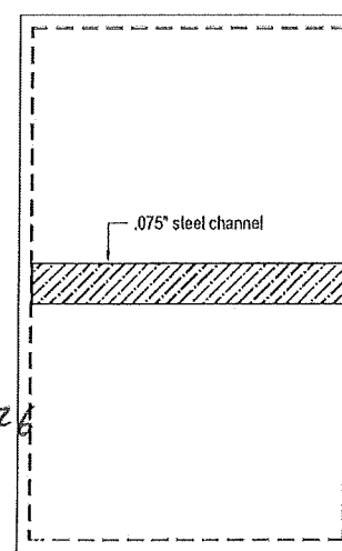
48" X 79" DOOR LEAF SHOWING INTERIOR CHANNEL REINFORCEMENT
