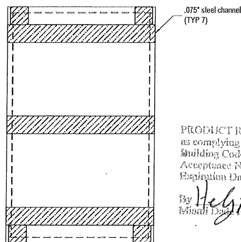
48" X 79" DOOR LEAF SHOWING EXTERIOR CHANNEL REINFORCEMENT
