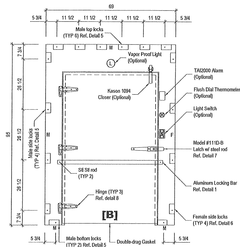
LOCKING BAR
