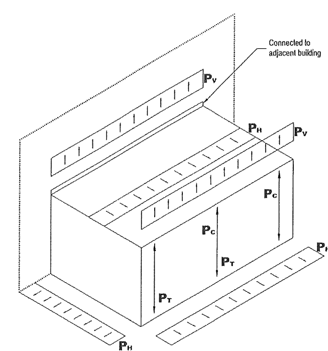
D ISOMETRIC WITH FOUNDATION WIND LOADS N.T.S.
