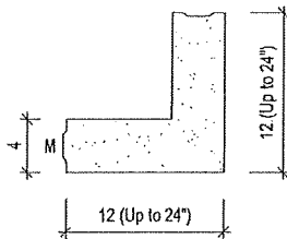
WC WALL PANEL (CORNER SECTION) SCALE: 1" = 1'-0"
