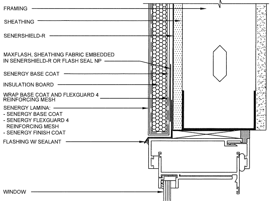
WINDOW HEAD (FLUSH)
