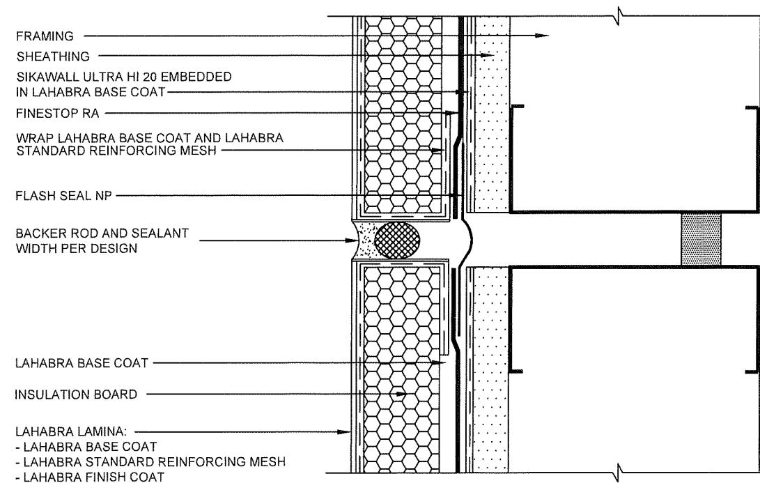
EXPANSION JOINT DETAIL PLAN VIEW
