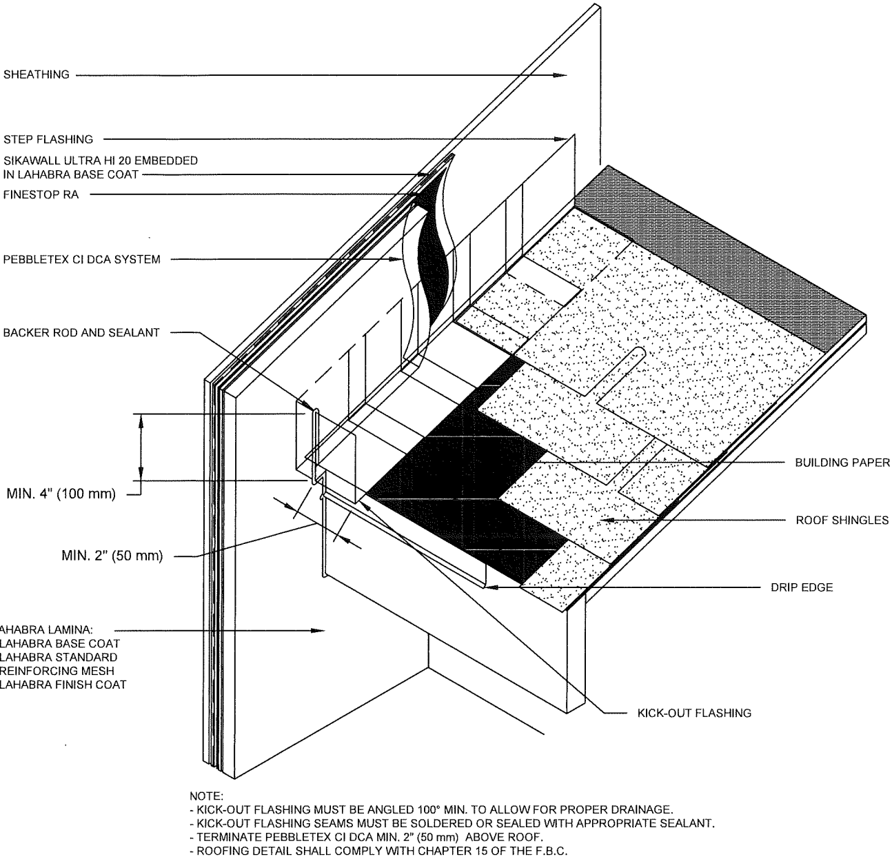
KICKOUT FLASHING DETAIL
