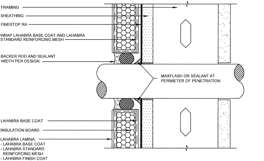
PIPE PENETRATION
