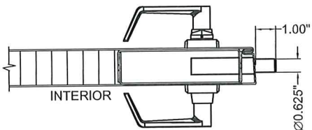
2 4 HORIZONTAL CROSS SECTION AWDCH SERIES LOCKSETS SINGLE DOORS
