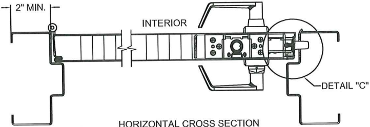
1 4 HORIZONTAL CROSS SECTION AWDCH & AWDCHJ SERIES LOCKSETS SINGLE DOORS
