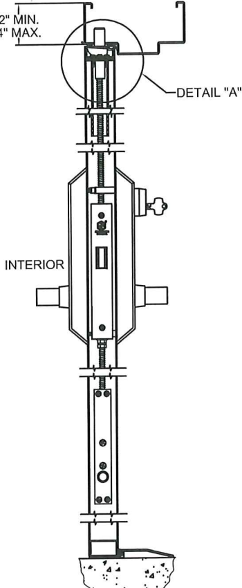
3 4 VERTICAL CROSS SECTION SINGLE DOOR HDWE AUTOBOLT-MAX AWDCH-EXX SERIES LOCK
