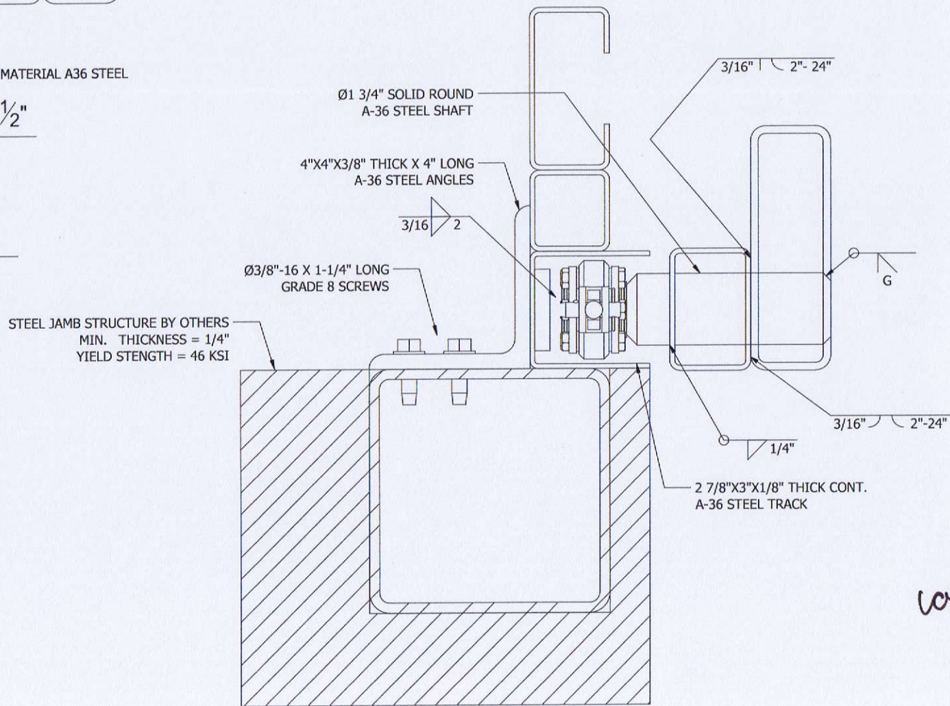
02 TRACK WELD DETAIL TYP.
