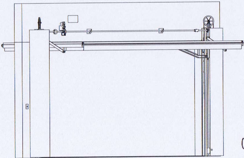
DOOR IN OPEN POSITION
