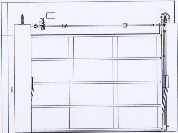
DOOR IN CLOSED POSITION
