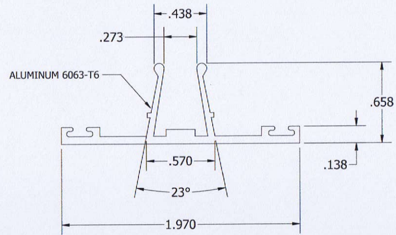
02 GLAZING BEAD (CAP)
