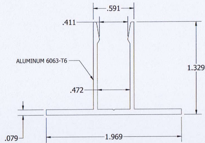
01 GLAZING BEAD (BASE)
