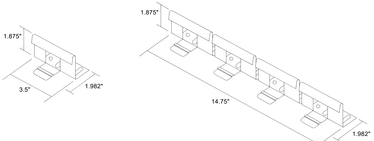
INDIVIDUAL CLIP
