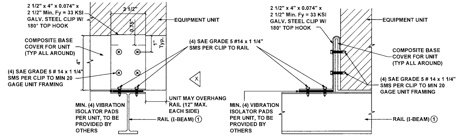
① CLIPPED UNIT CONNECTION SCALE: 1/4" = 0'-1" ELEVATION
