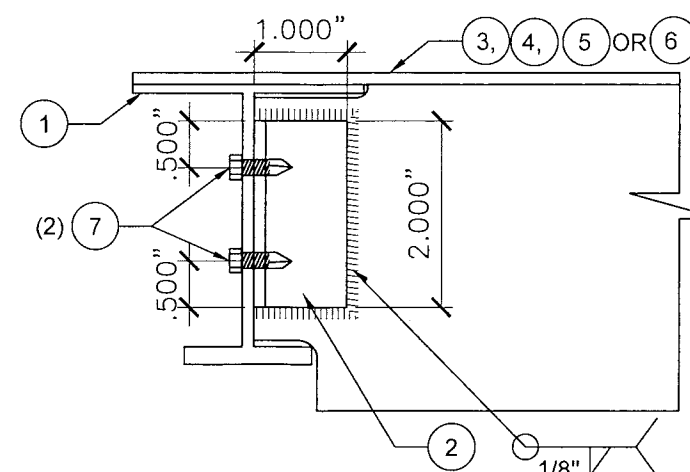
DETAIL 3: (PARTIALLY ON TOP OF 1)
