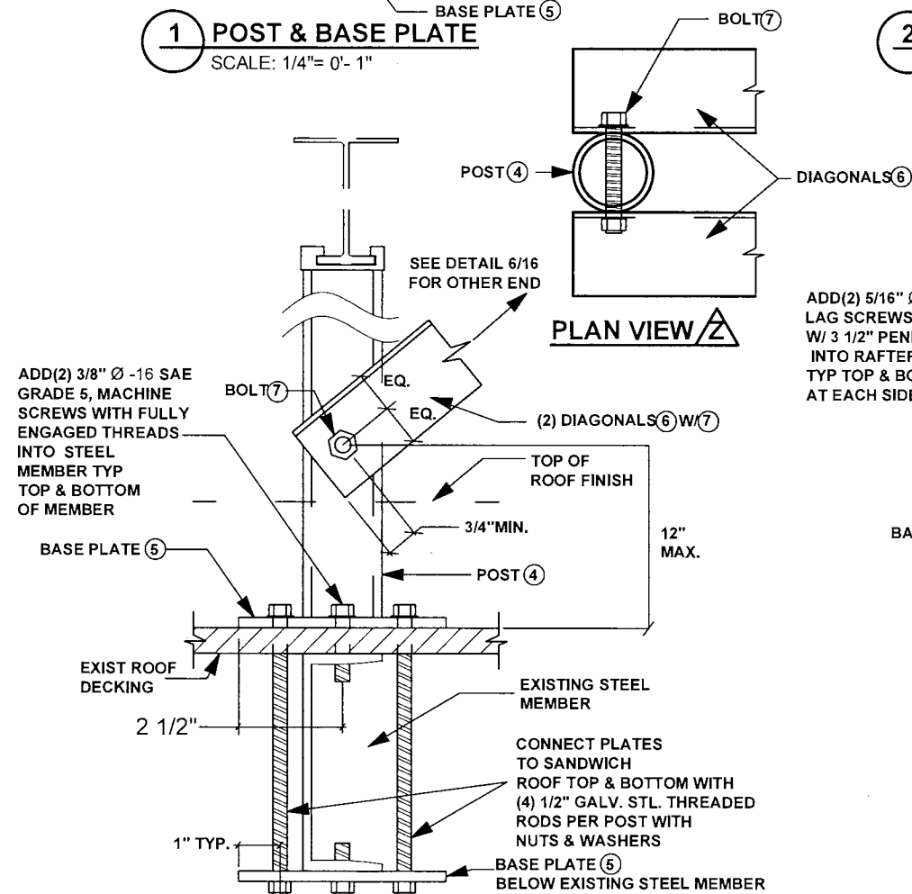
4 BASE PLATE ATTACHMENT TO EXISTING STEEL TRUSS OR STEEL BEAM ROOF SCALE: 1/4"= 0'- 1" ELEVATION
