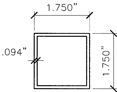
②A LARGE STRUT TUBING 1/2"= 0'- 1"
