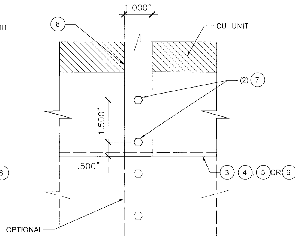
VIEW U
