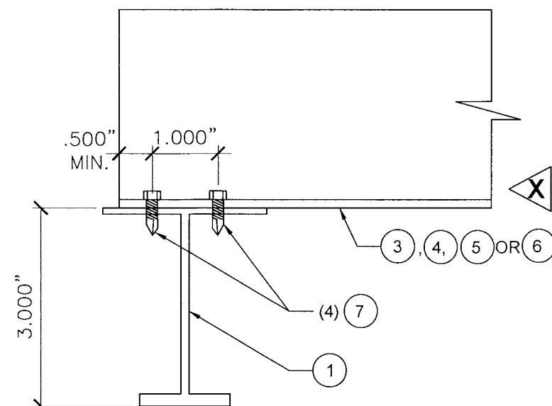
DETAIL 1: (ON TOP OF 1)
