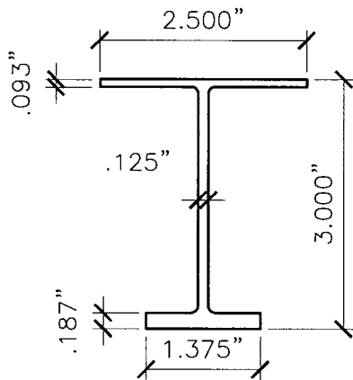
① RAIL ( I-BEAM) 1/2"= 0'- 1"
