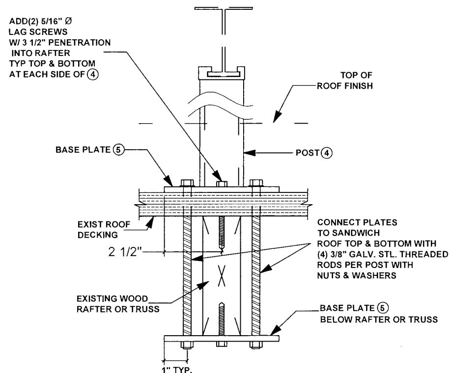
5 BASE PLATE ATTACHMENT TO EXISTING WOOD TRUSS OR WOOD RAFTER ROOF SCALE: 1/4"= 0'- 1" ELEVATION
