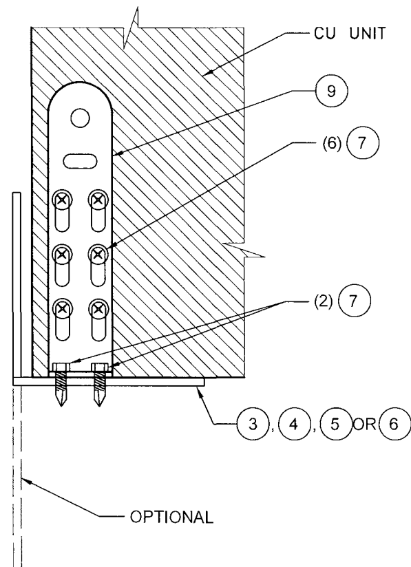
DETAIL 4 1/2"= 0'- 1" ELEVATION
