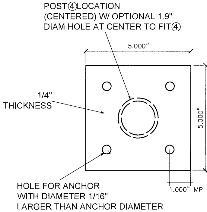
⑤ BASE PLATE 3/8"= 0'- 1"
