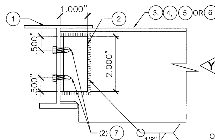
DETAIL 2: (BELOW TOP OF 1)
