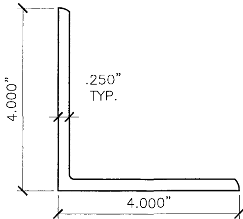
⑥ CROSS BAR 1/2"= 0'- 1"
