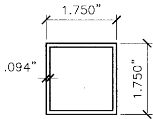
②A LARGE STRUT TUBING 1/2"= 0'- 1"
