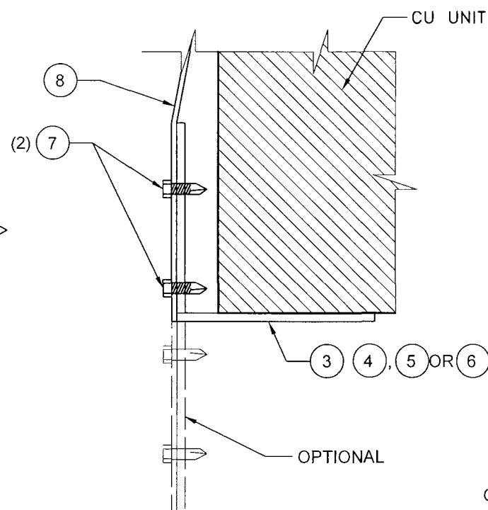
DETAIL 5 1/2"= 0'- 1" ELEVATION
