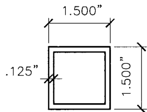
②B SMALL STRUT TUBING 1/2"= 0'- 1"
