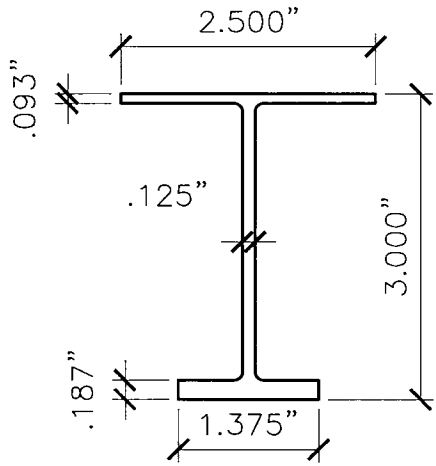
① RAIL ( I-BEAM) 1/2"= 0'- 1"
