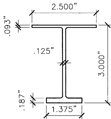
① RAIL ( I-BEAM) 1/2"= 0'- 1"
