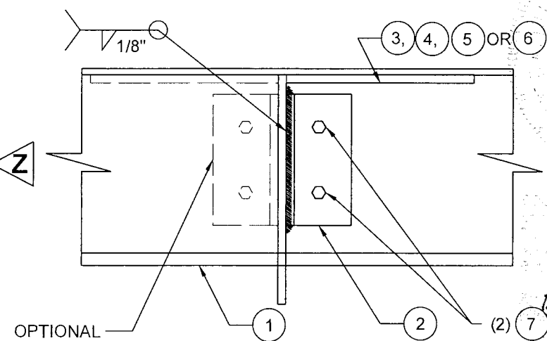
VIEW Z
