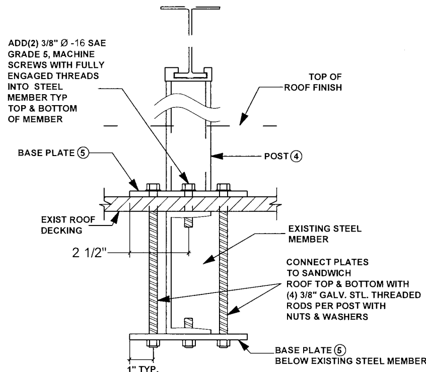
4 BASE PLATE ATTACHMENT TO EXISTING STEEL TRUSS OR STEEL BEAM ROOF SCALE: 1/4"= 0'- 1" ELEVATION
