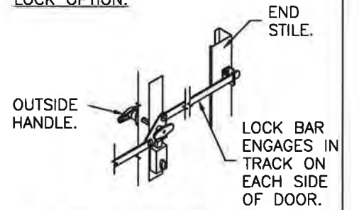
OUTSIDE KEYPED LOCK WITH LOCK BAR LOCKING.
