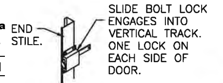
INSIDE SLIDE BOLT LOCK OPTION.
