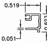
87 1/4" STOP N.T.S. 6063-T6 VERTICAL
