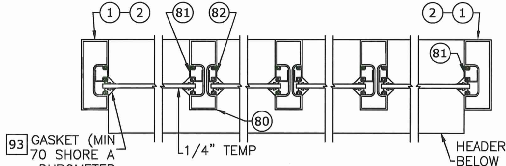
NON-IMPACT TRANSOM GLAZING DETAILS NTS 1/4" TEMPERED H SECTION BI-PARTING
