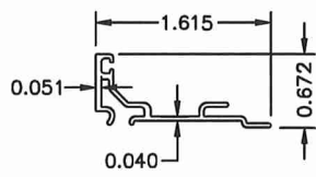
86B IG GUTTER N.T.S. 6063-T6 ALTERNATIVE 2 (NEW)
