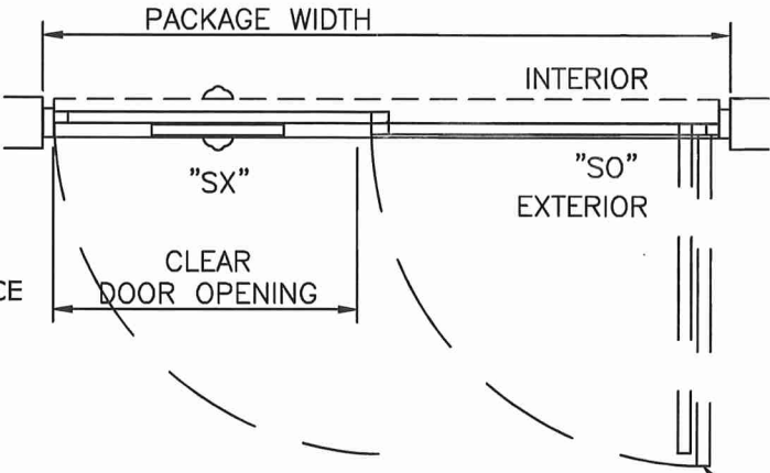
SERIES 3000 (SX-SO) SINGLE SLIDE PLAN
