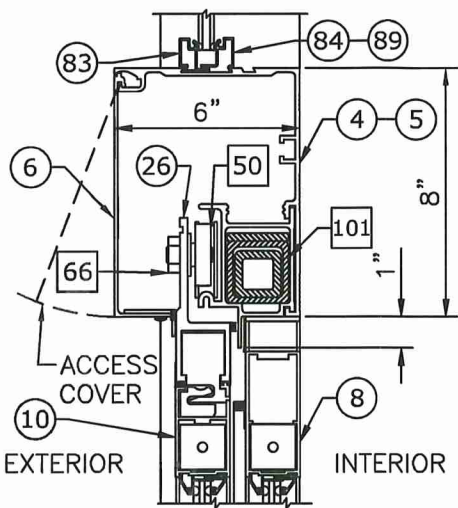
①A VERTICAL SECTION 2"=1'-0" BI-PARTING HEADER REINFORCING DETAIL WITH TRANSOM
