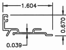
86A IG GUTTER N.T.S. 6063-T6 ALTERNATIVE 1 (ORIGINAL)
