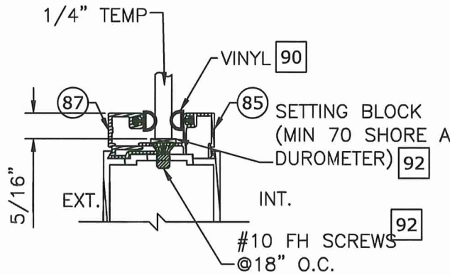
NON-IMPACT DOOR PANEL GLAZING DETAILS NTS SERIES 2000/3000
