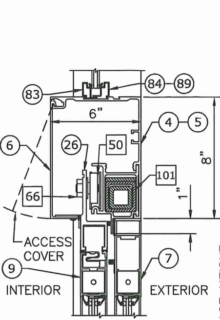
5A VERTICAL SECTION 2"=1'-0" BI-PARTING HEADER REINFORCING DETAIL WITH TRANSOM
