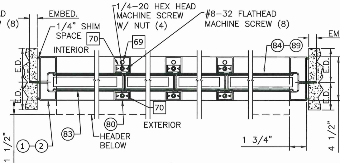
14 SERIES 2000/3000 TRANSOM 2"=1'-0" BI-PARTING
