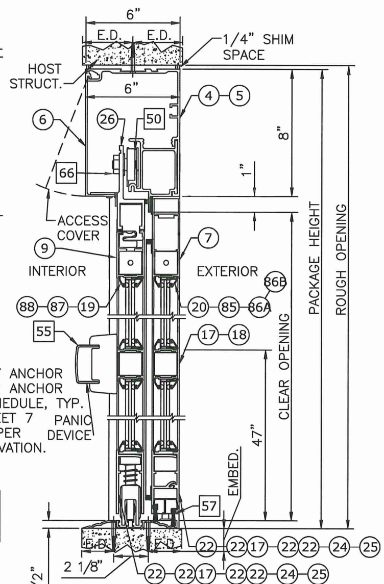
6 VERTICAL SECTION 2"=1'-0"
