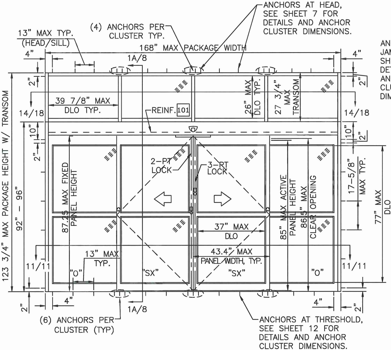
DURA-STORM 2000 TYPICAL ELEVATIONS
