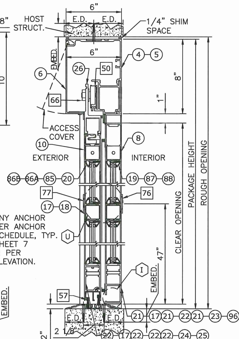
② VERTICAL SECTION 2"=1'-0"
