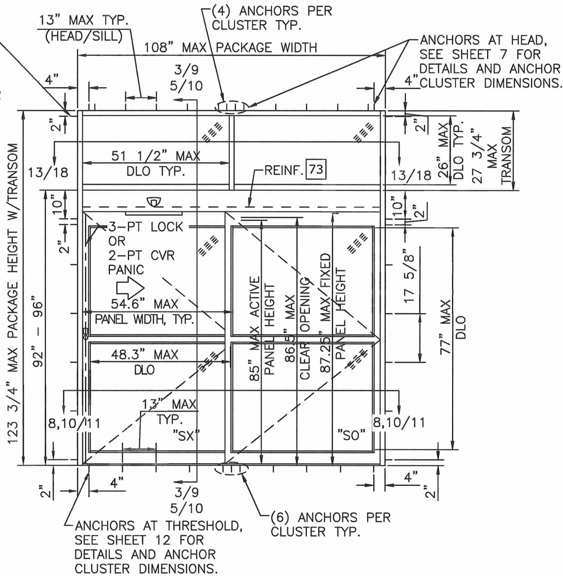
DURA-STORM 3000 TYPICAL ELEVATIONS
