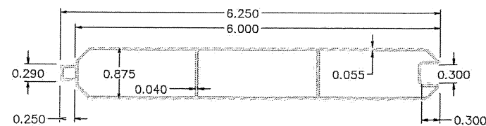
6" PVC PICKET
