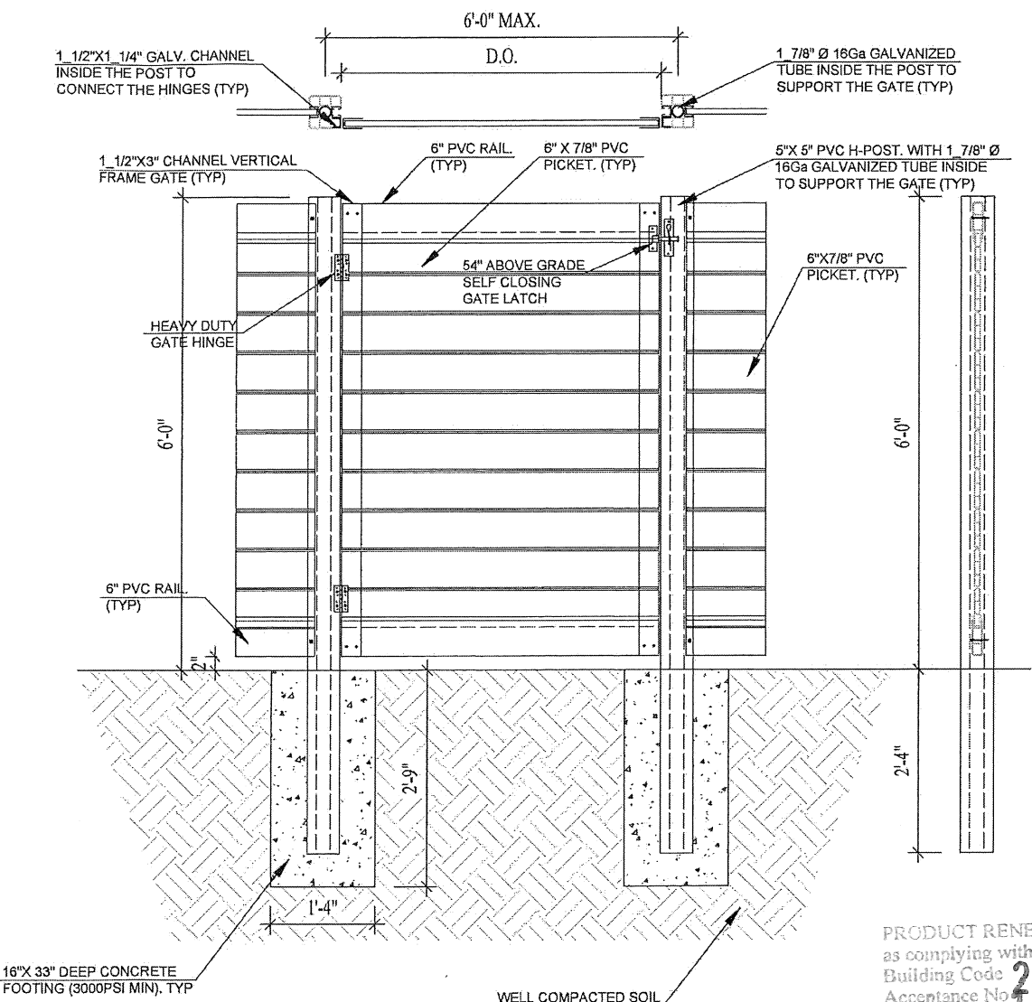
2 SINGLE GATE N.T.S. ELEVATION VIEW
