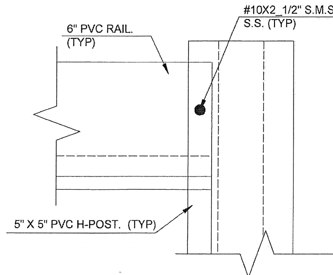
8 CONNECTION RAIL-POST TYP
