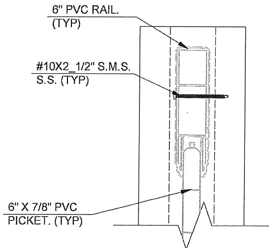
9 CONNECTION RAIL-PICKETS TYP
