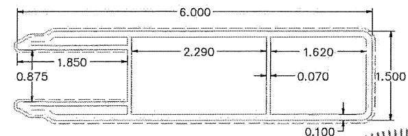
6" PVC RAIL
