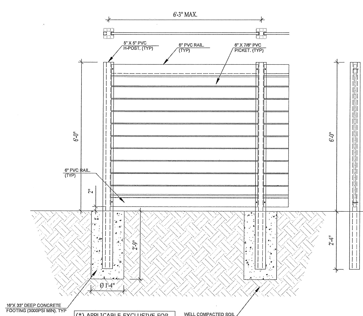
1 PVC FENCE N.T.S. ELEVATION VIEW
