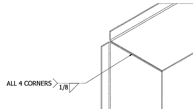
UNIVERSAL SLEEVE CORNER WELDS
