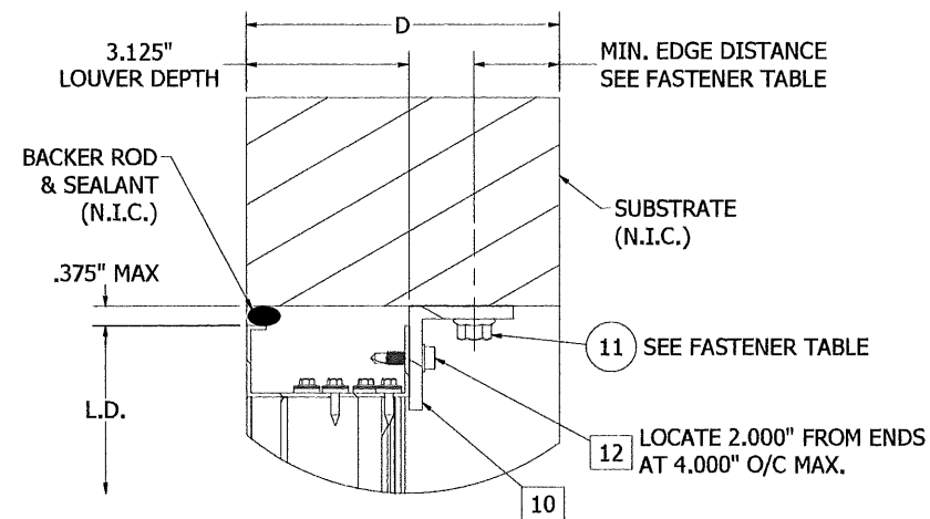
DETAIL 4 RETAINING ANGLE INSTALL AT HEAD
