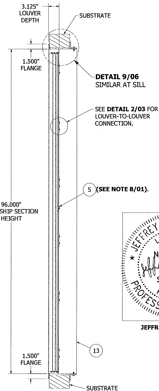
SECTION C-C
