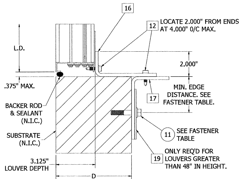
DETAIL 7 DOUBLE ANGLE INSTALLED AT SILL
