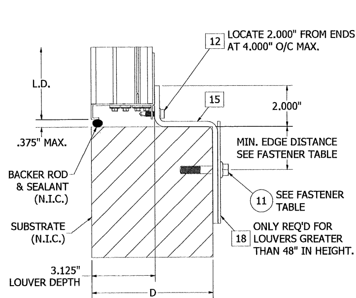
DETAIL 5 RETAINING ZEE INSTALLED AT SILL
