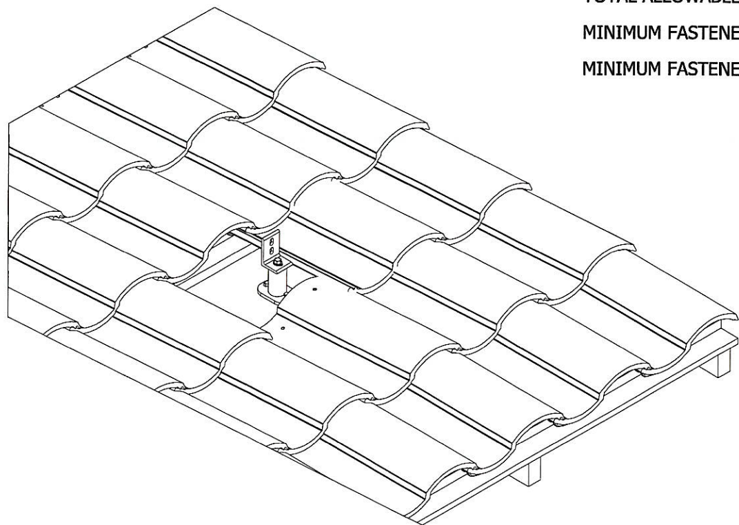
TILE REPLACEMENT INSTALLATION NOT TO SCALE
