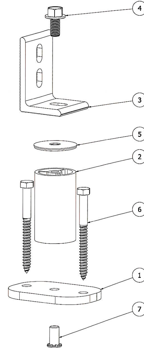
EXPLODED VIEW
