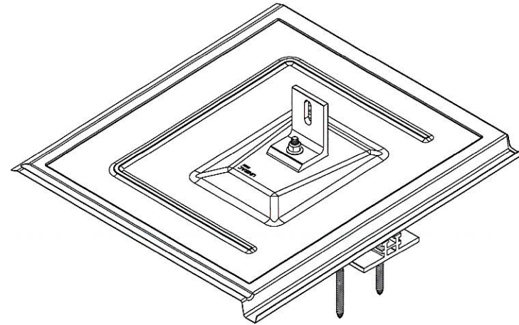
FLAT TILE REPLACEMENT ASSEMBLY
