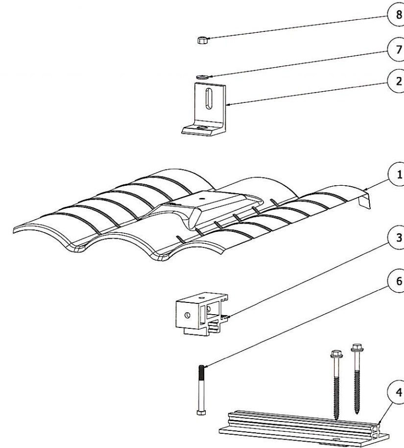
EXPLODED VIEW
