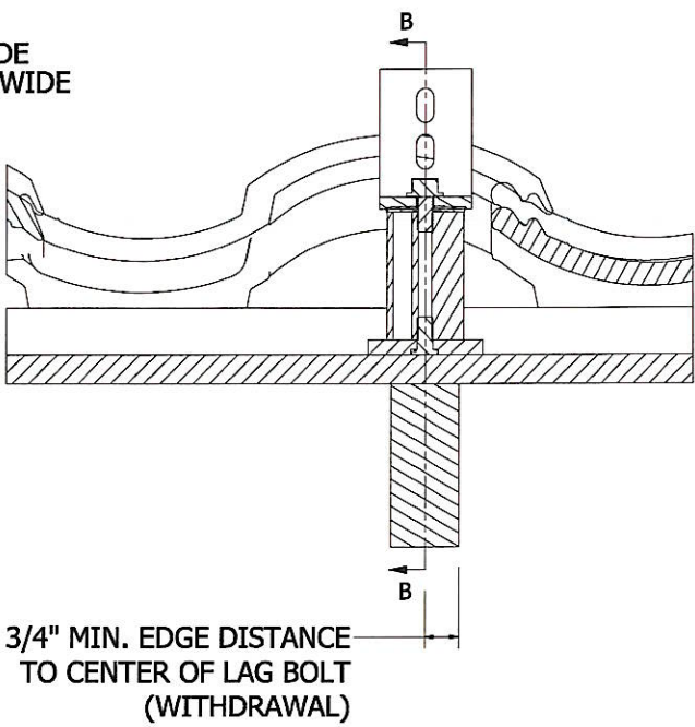
SECTION STAND OFF ATTACHMENT NOT TO SCALE
