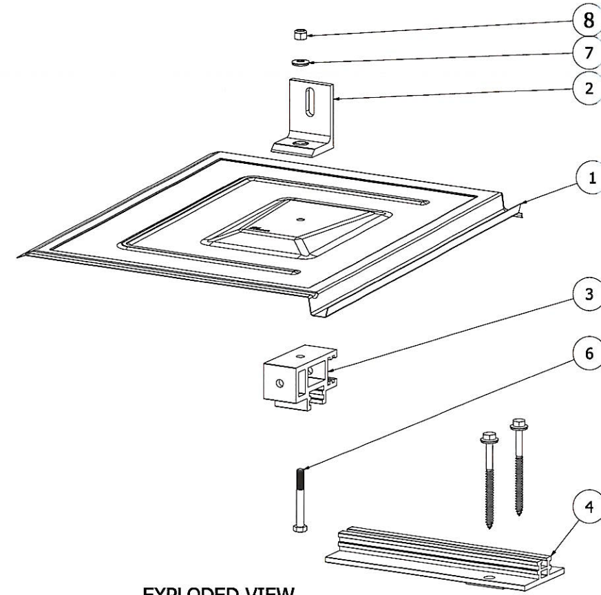
EXPLODED VIEW
