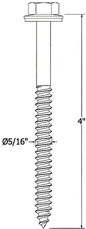
ITEM 3 LAG SCREW EPDM WASHER ASSEMBLY
