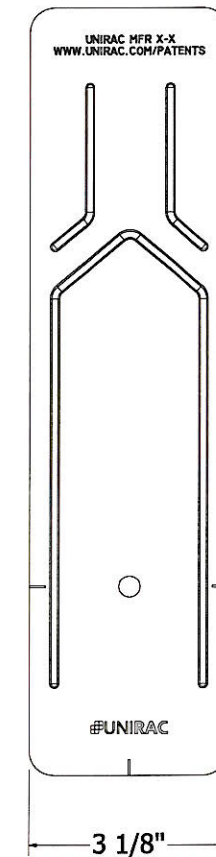
ITEM 1 3 INCH FLASHING
