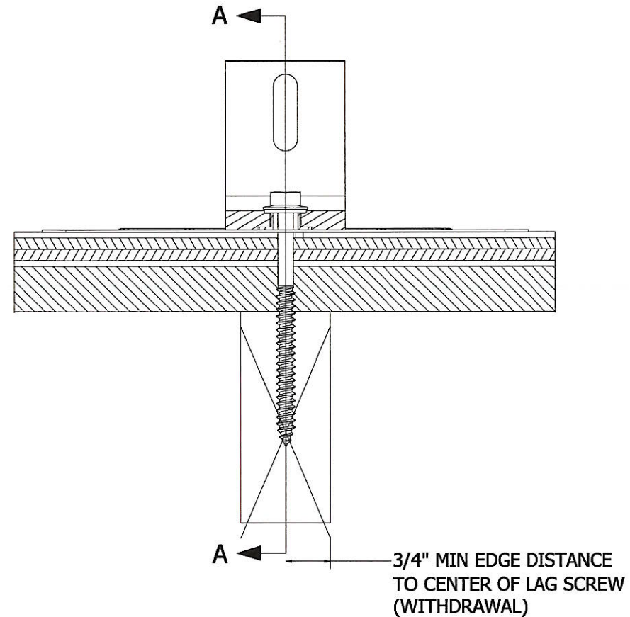
SECTION L-FOOT FLASHING DETAIL NOT TO SCALE
