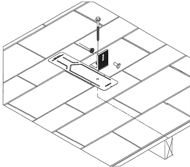
ALTERNATE L-FOOT CONFIGURATION NOT TO SCALE
