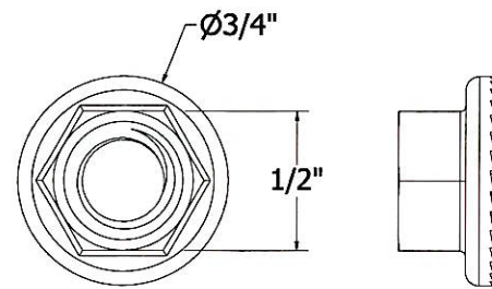
ITEM 5 3/8-16 SERRATED FLANGE NUT
