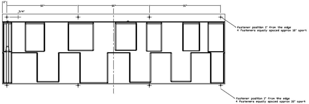
DECRA COLONIAL SHINGLE FIELD CONDITION FASTENING PATTERN
