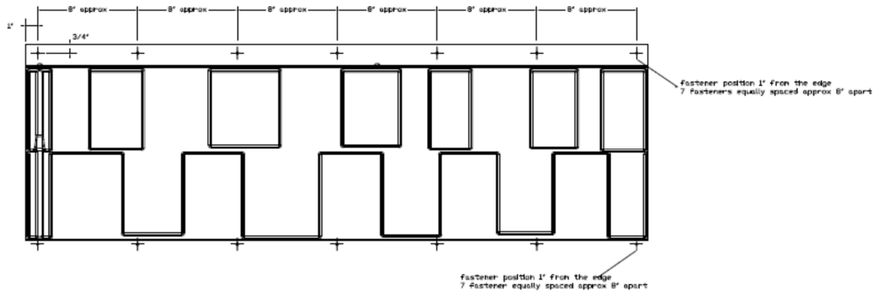
DECRA COLONIAL SHINGLE PERIMETER AND CORNER CONDITION FASTENING PATTERN
