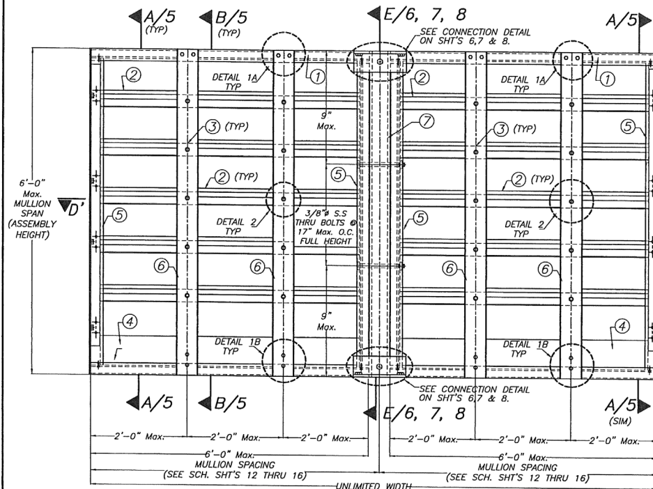
MULTIPLE UNITS HORIZONTALLY EXPANDED (INTERIOR ELEVATION)
