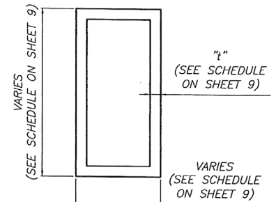
⑦ MULLION 6063-T6 ALLOY SCALE: 3/8"=1"
