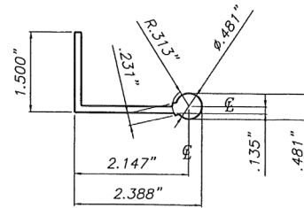
③ 4" BLADE SUPPORT SCALE: 3/8"=1"
