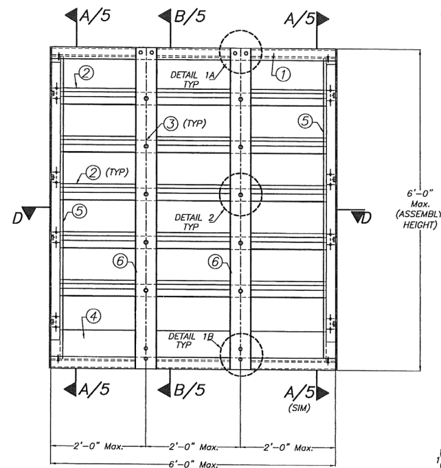
SINGLE UNIT (INTERIOR ELEVATION)
