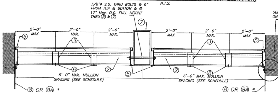
MULTIPLE UNITS HORIZONTALLY EXPANDED (INTERIOR ELEVATION)
