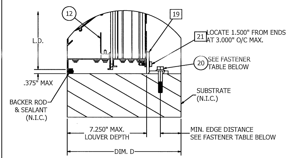
DETAIL 3 ANGLE INSTALL AT SILL
