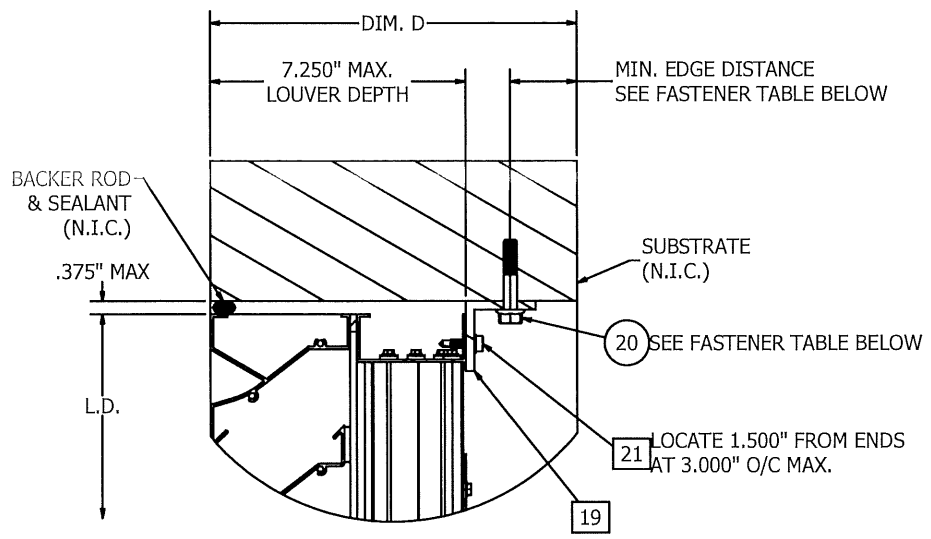
DETAIL 4 ANGLE INSTALL AT HEAD
