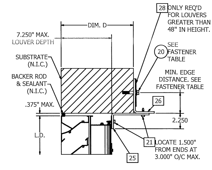
DETAIL 8 DOUBLE ANGLE INSTALLED AT HEAD
