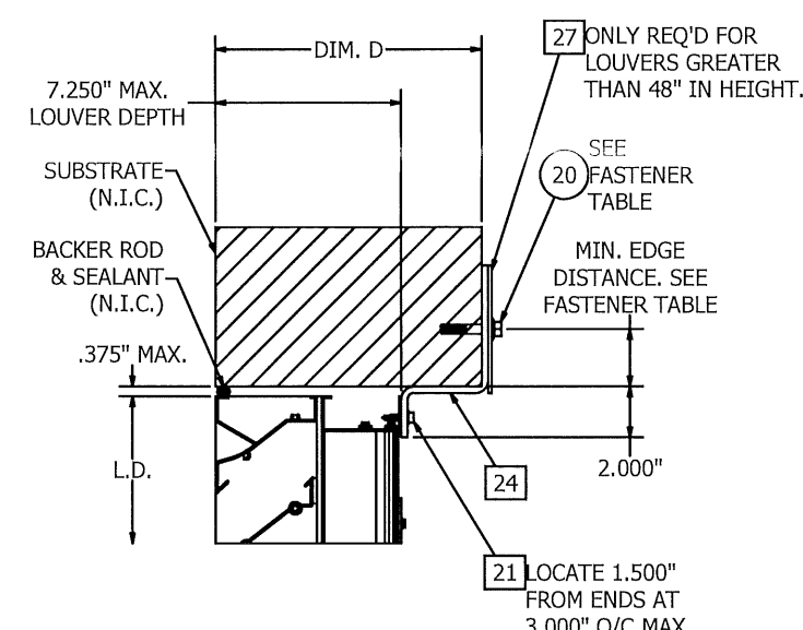
DETAIL 6 RETAINING ZEE INSTALLED AT HEAD
