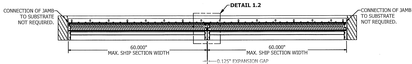
SECTION B-B
