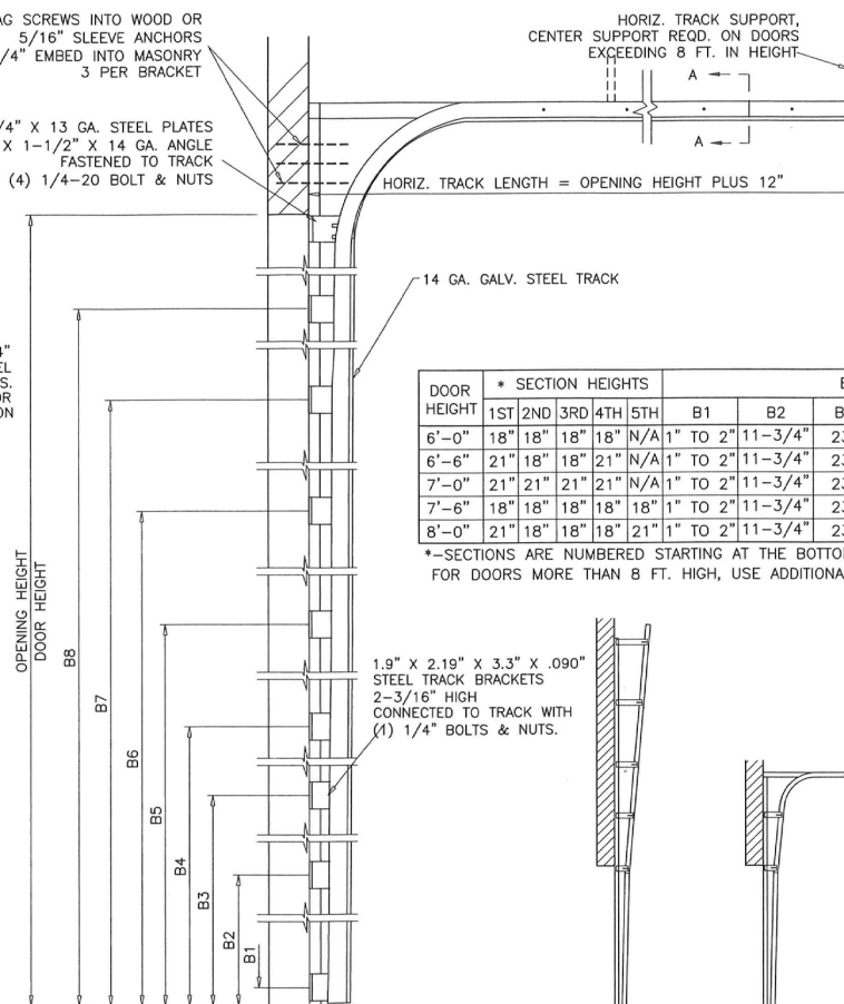
TRACK CONFIGURATION
