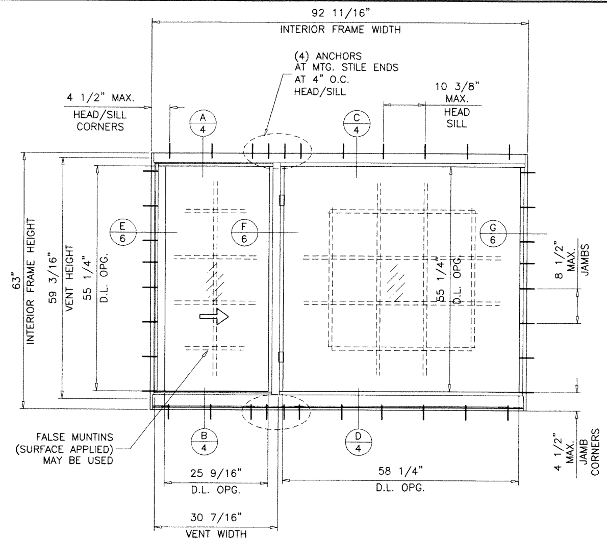
TYPICAL ELEVATIONS
