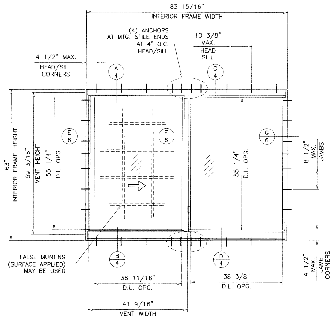
TYPICAL ELEVATIONS
