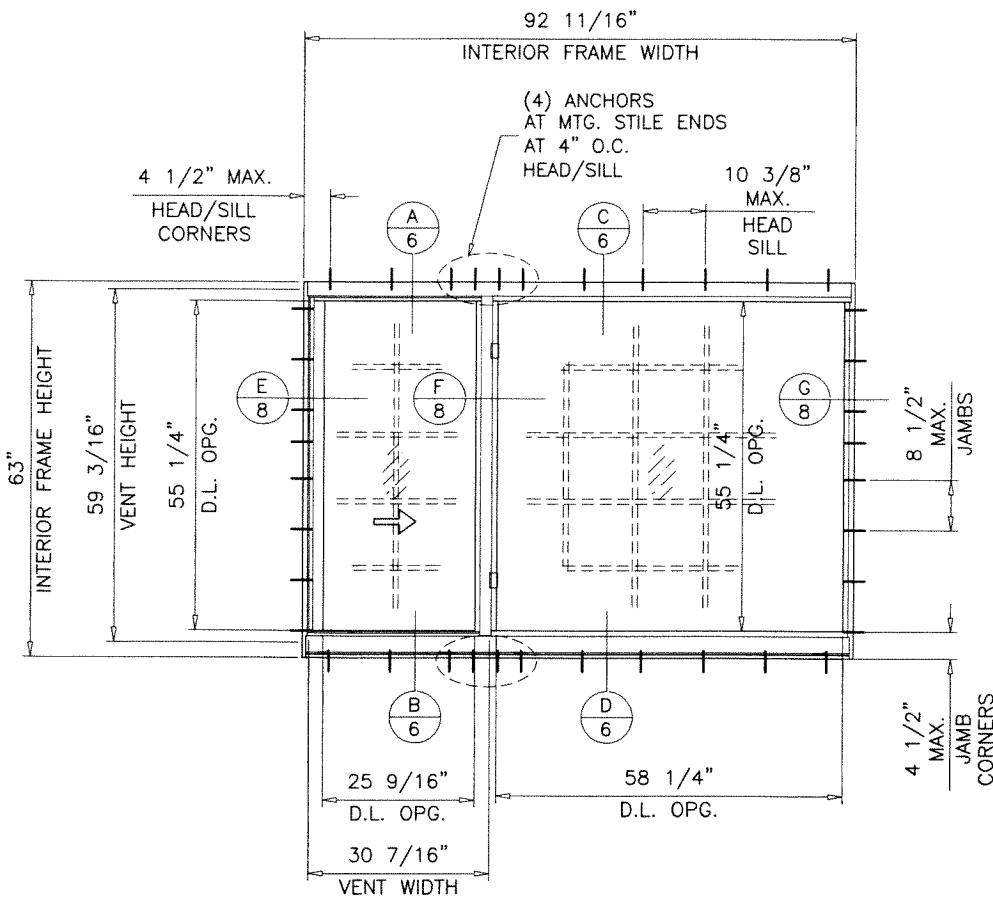
TYPICAL ELEVATIONS (UNEQUAL LITES)
