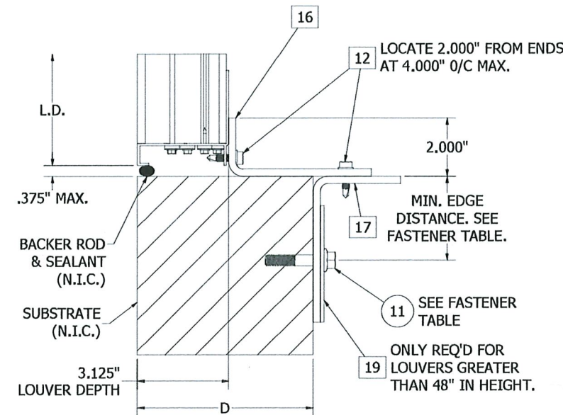
DETAIL 7 DOUBLE ANGLE INSTALLED AT SILL
