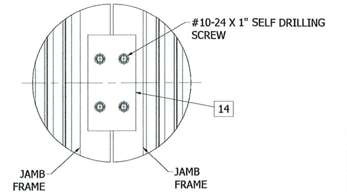
DETAIL 2 LOUVER-TO-LOUVER SPLICE
