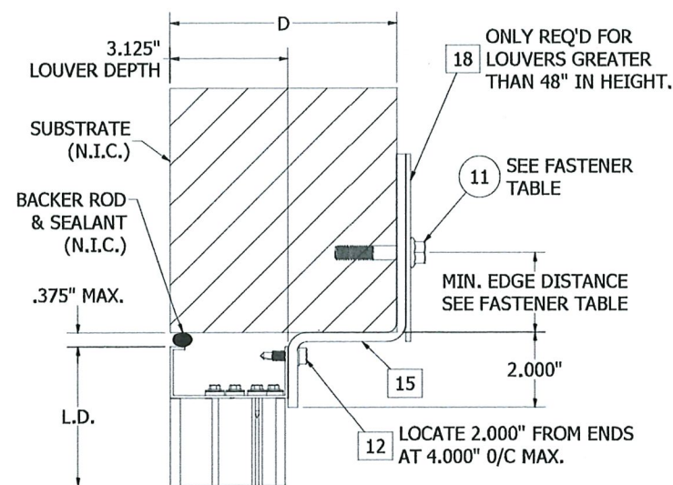
DETAIL 6 RETAINING ZEE INSTALLED AT HEAD
