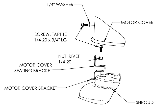
MOTOR COVER MOUNTING WITH SHROUD
