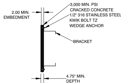
CONCRETE DECK ANCHORING
