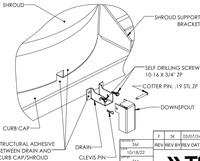
DRAIN & DOWNSPOUT MOUNTING SIZE 177- 197
