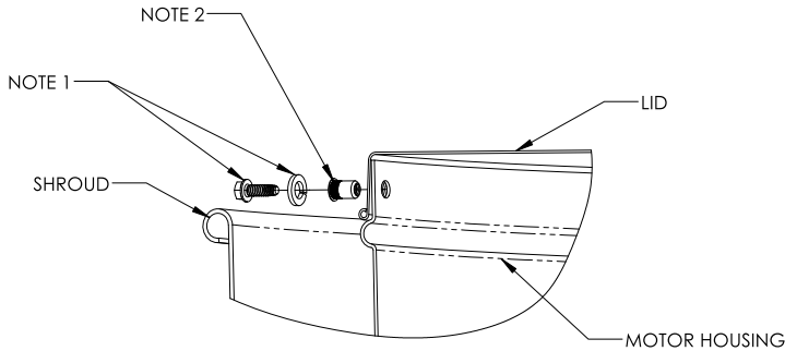
LID MOUNTING ON MOTOR HOUSING SIZE 177 - 197
