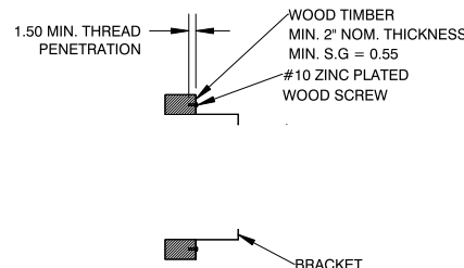
TIMBER ANCHORING
