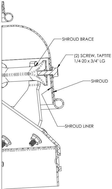
SHROUD MOUNTING WITH SHROUD BRACE
