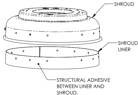
SHROUD LINER STRUCTURAL ADHESIVE INSIDE SHROUD
