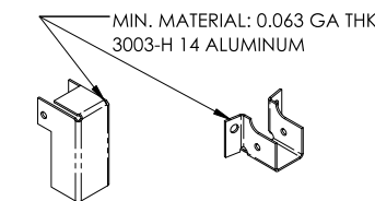
DRAIN
