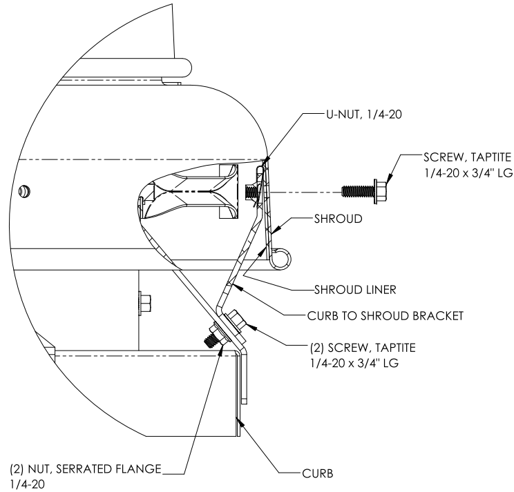
SHROUD MOUNTING WITH CURB SHROUD SUPPORT BRACKET
