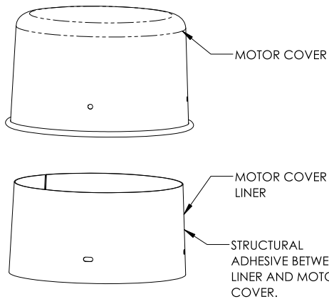
MOTOR COVER LINER STRUCTURAL ADHESIVE INSIDE MOTOR COVER
