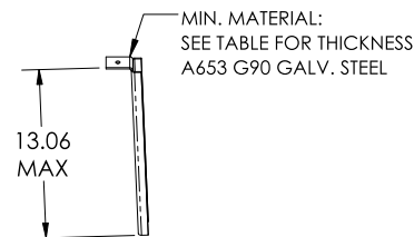
VERTICAL SUPPORT POST
