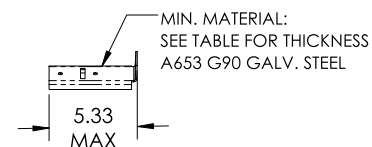
HORIZONTAL SUPPORT POST
