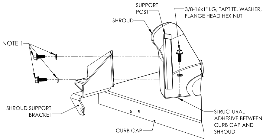
SHROUD BRACKET MOUNTING WITH SHROUD & SUPPORT POST SIZE 177- 197
