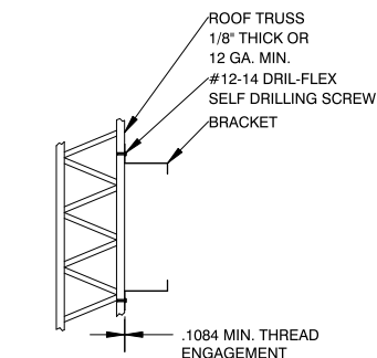
STEEL ANCHORING
