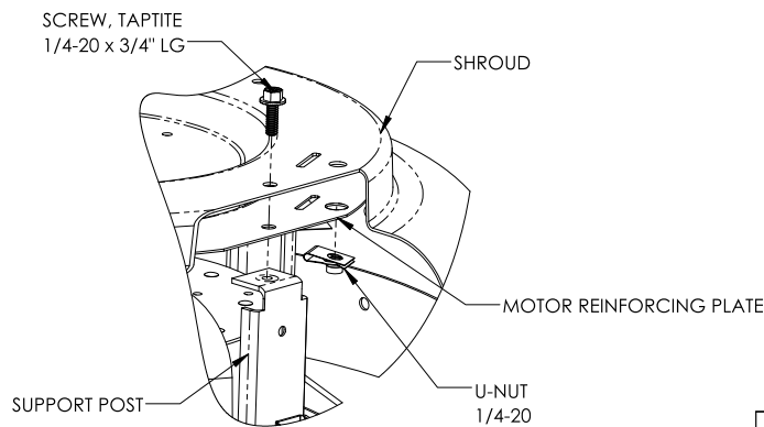
SUPPORT POST MOUNTING WITH SHROUD & DECK PLATE
