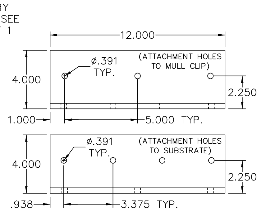
(158) 4x4x3/8" ALUMINUM MOUNTING ANGLE @ MULLS
