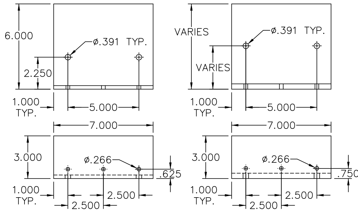
(157) 3x6x1/4" ALUMINUM
