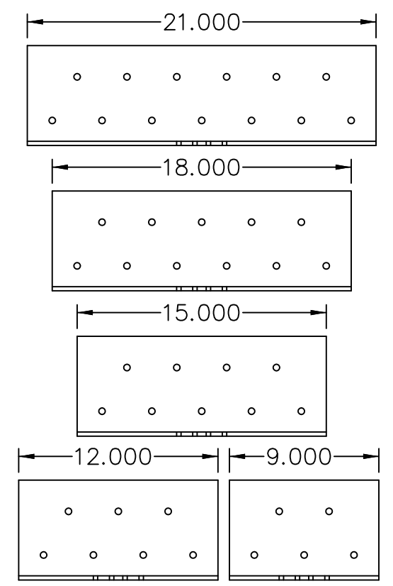
(157) MULL CLIP TO SUBSTRATE ALTERNATE SIZE LAYOUTS (FOLLOW SAME EDGE / HOLE SPACING AS 24")
