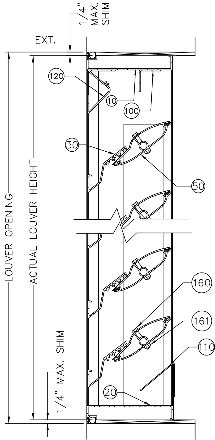
A 3 VERTICAL SECTION DETAIL
