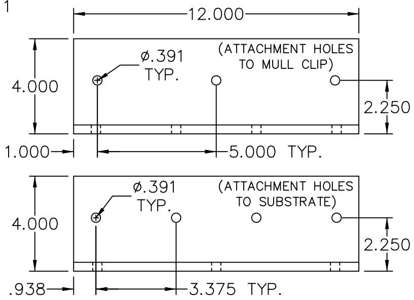
(158) 4x4x3/8" ALUMINUM MOUNTING ANGLE @ MULLS
