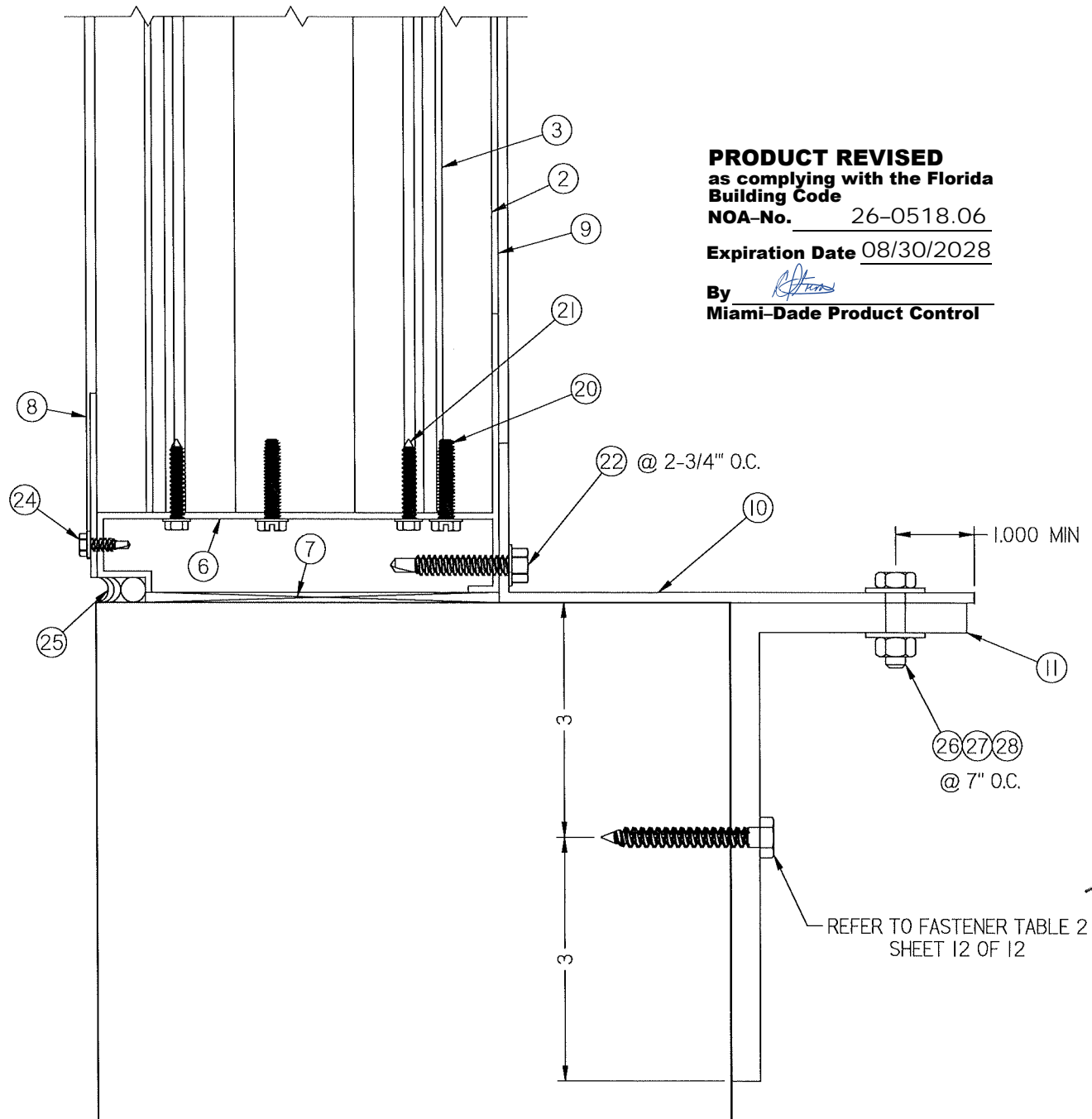
SILL DETAIL SKINNY WALL 2B 5/12
