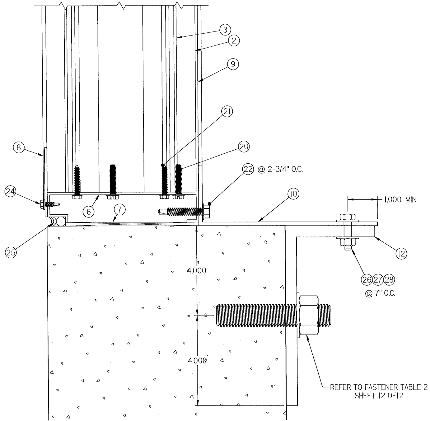
SILL DETAIL SKINNY WALL 2A 5/12
