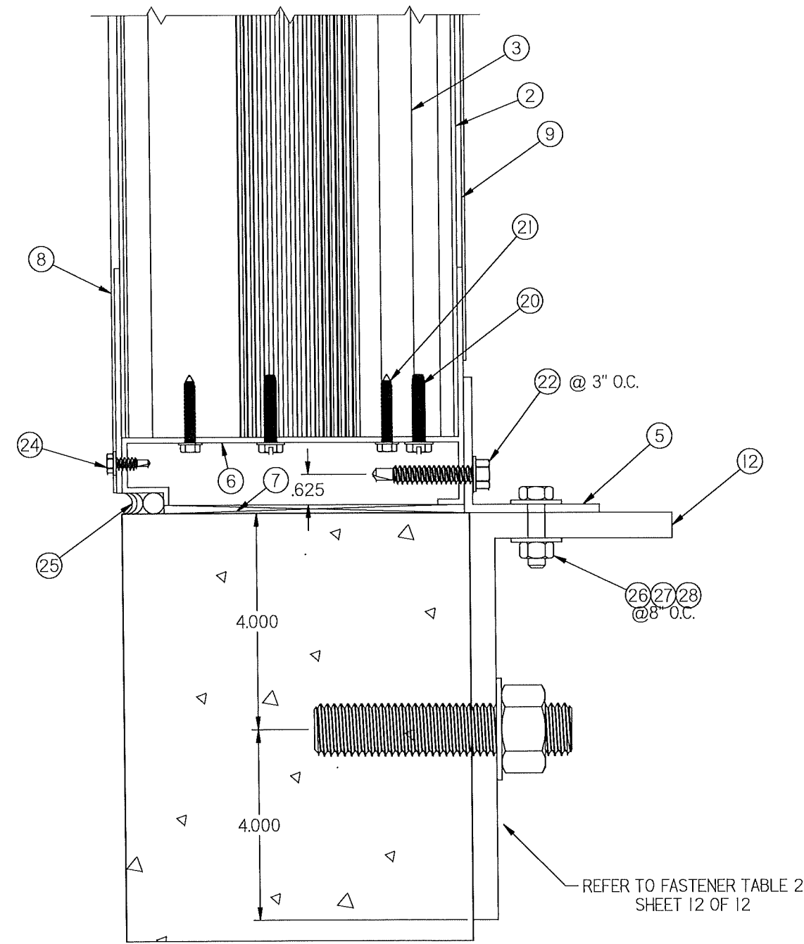
SILL DETAIL 2A SKINNY WALL 4/12
