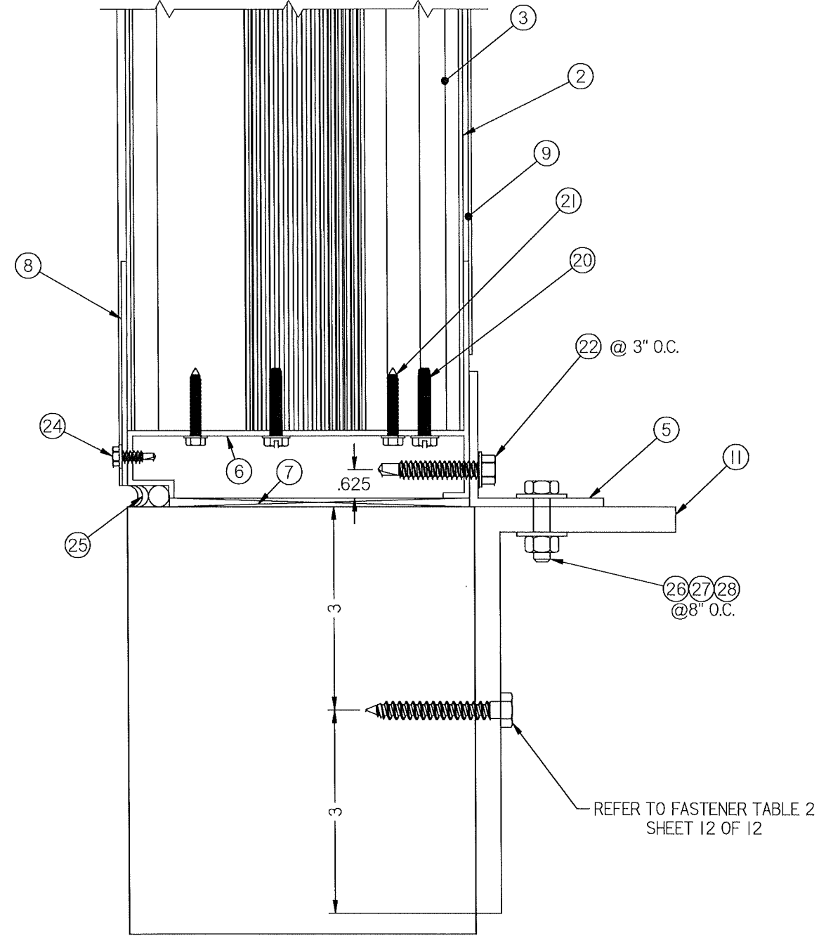
SILL DETAIL 2B SKINNY WALL 4/12
