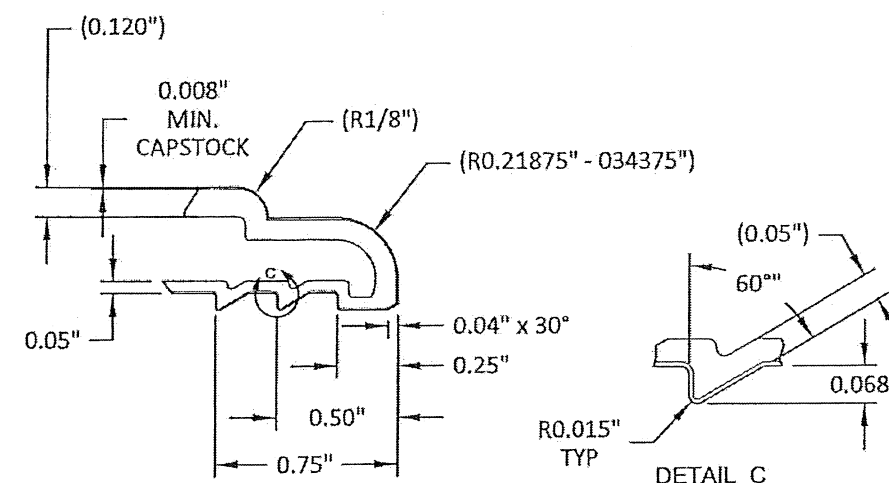
B 2 DETAIL 2' X 6-1/2" SLOTTED RIBBED SLOTTED RAIL PVC
