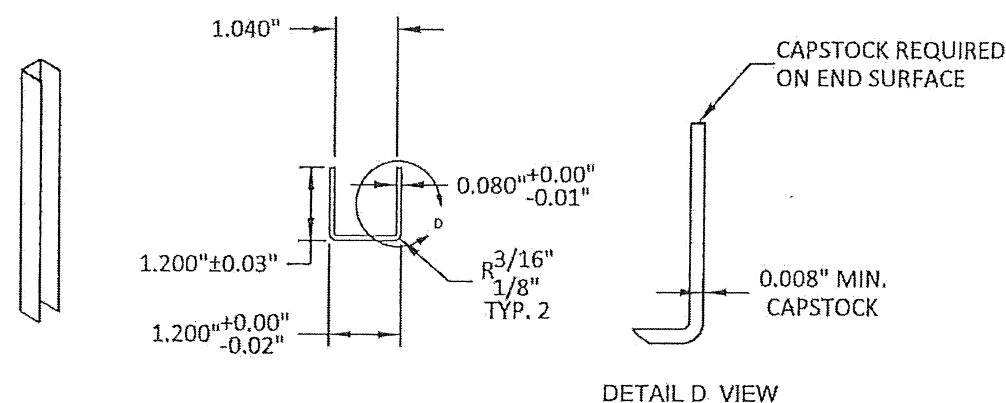
A 2 DETAIL 5" X 5" RW POST PVC
