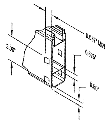
DETAIL OF NOTCHES
