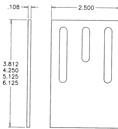
TRACK PLATE 12 GA. STEEL
