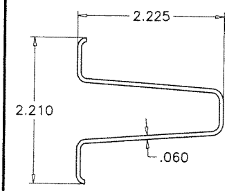
REINF. TRUSS 16 GA. STEEL
