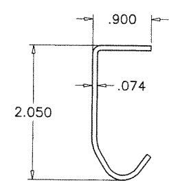
TRACK 14 GA. STEEL
