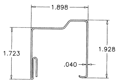
TOP RAIL 20 GA. STEEL
