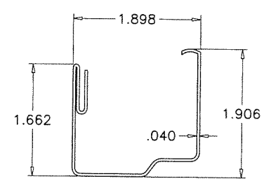
BOTTOM RAIL 20 GA. STEEL
