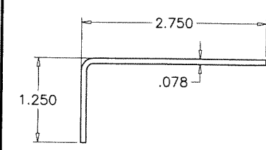
TRACK ANGLE 14 GA. STEEL
