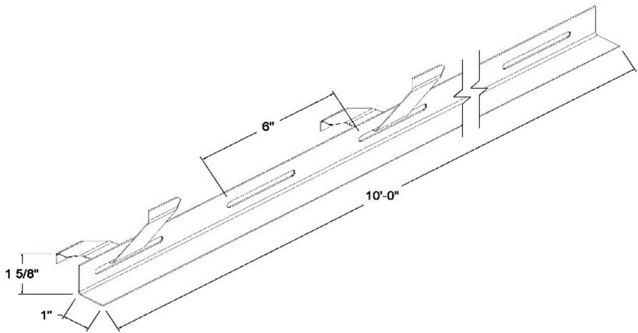
PAC-150 CONTINUOUS BUTTERFLY CLIP
