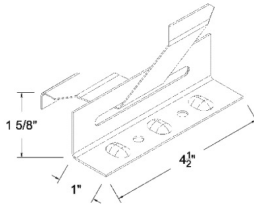
PAC-150 BUTTERFLY CLIP
