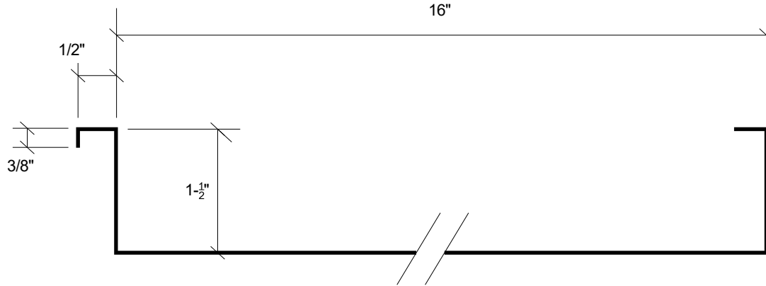
PAC-150 – 24GA. STEEL PANEL
