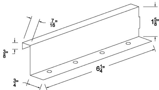
22 GA, PAC-150 FIXED CLIP
