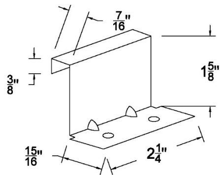
24 GA, PAC-150 FIXED CLIP
