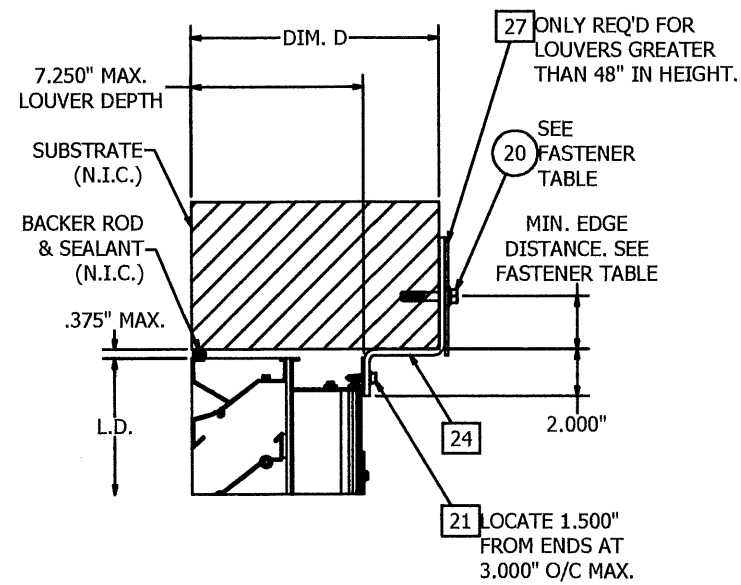
DETAIL 6 RETAINING ZEE INSTALLED AT HEAD
