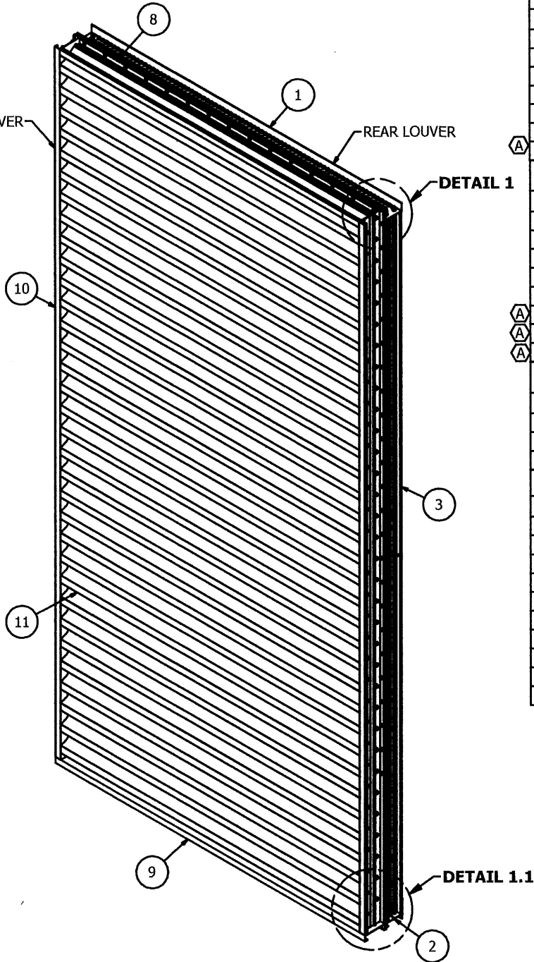
700HZDC COMBINATION RECTANGLE LOUVER N.T.S. (CF) 60"W X 120"H SHOWN
