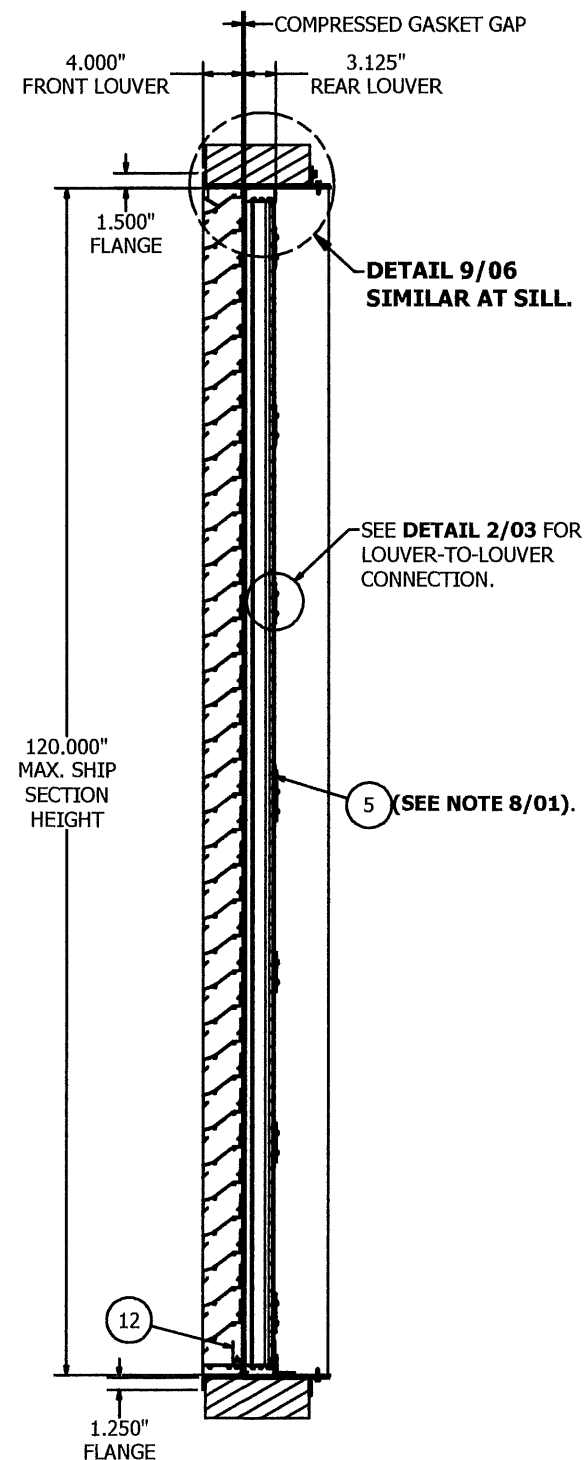
SECTION C-C
