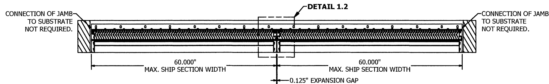
SECTION B-B
