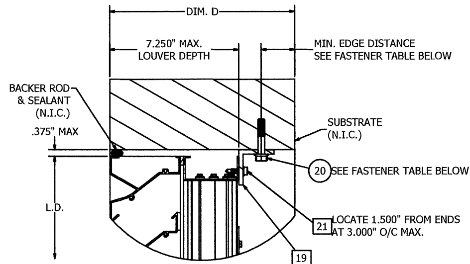
DETAIL 4 ANGLE INSTALL AT HEAD
