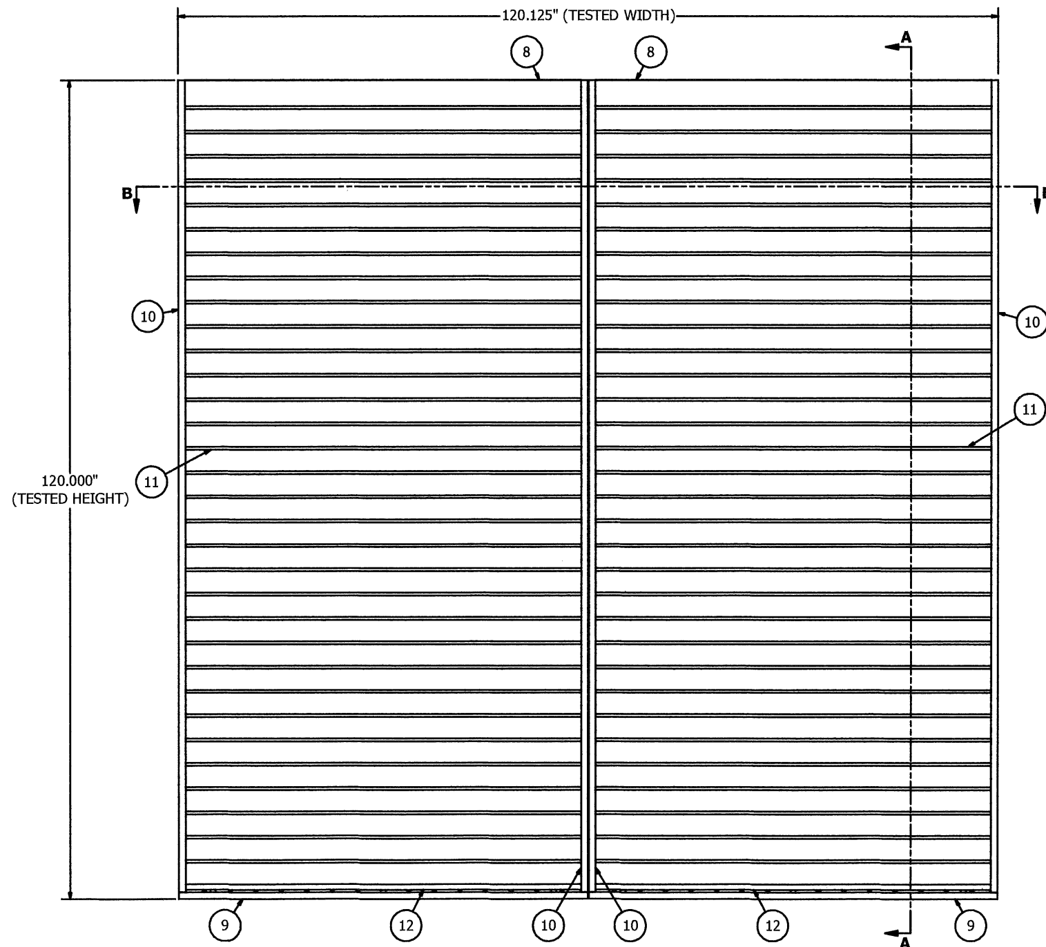
MULTI-SECTION ASSEMBLY - CHANNEL FRAME (FRONT) LOUVER
