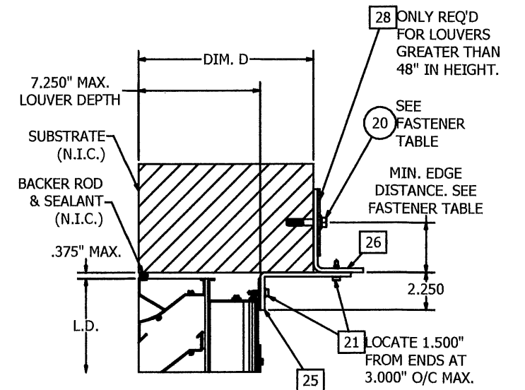
DETAIL 8 DOUBLE ANGLE INSTALLED AT HEAD
