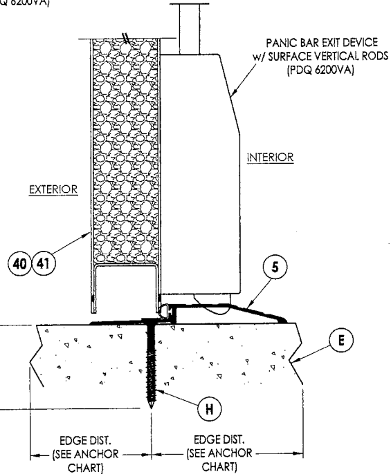
4 6 VERTICAL CROSS SECTION w/ SURFACE VERTICAL RODS
