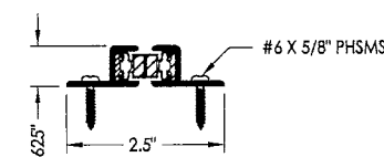
ASTRAGAL GASKET
