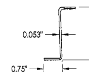
3 "Z" ASTRAGAL
