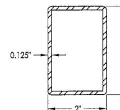
2 MULLION PDQ 9200M-11 SERIES
