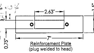
21 FLUSHBOLT FRAME REINFORCEMENT 16 GA STEEL
