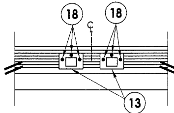
DETAIL 2 Vertical Surface Rod Strike Plate @ Sill
