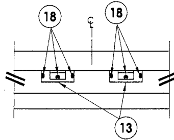
DETAIL 1 Vertical Surface Rod Strike Plate @ Head
