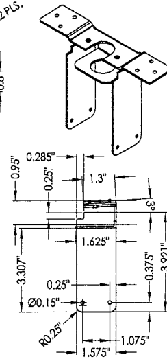
23 CYLINDRICAL LOCK REINFORCEMENT
