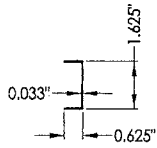
26 PERIMETER GLAZED CHANNEL REINFORCEMENT 20 GA. GALV. STEEL
