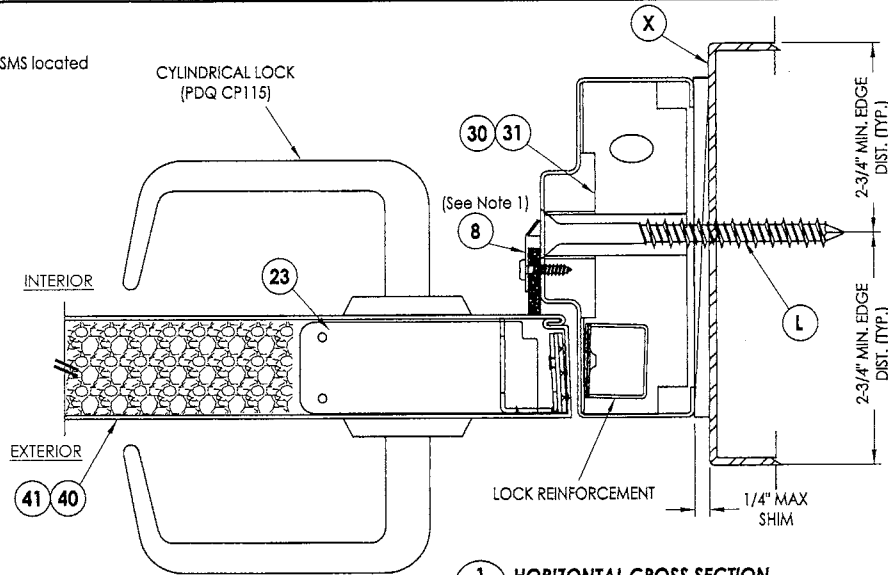
1 HORIZONTAL CROSS SECTION 4 CYLINDRICAL LOCK (PDQ)
