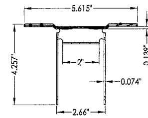
23 CYLINDRICAL LOCK REINFORCEMENT
