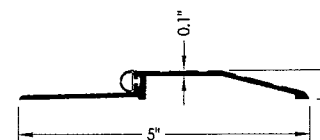
5 OUTSWING BUMP THRESHOLD HAGER 477S
