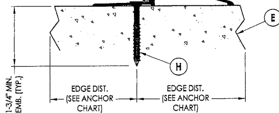
2 6 VERTICAL CROSS SECTION
