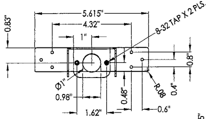
31 EMA BUTTERFLY ANCHOR 18 GA STEEL
