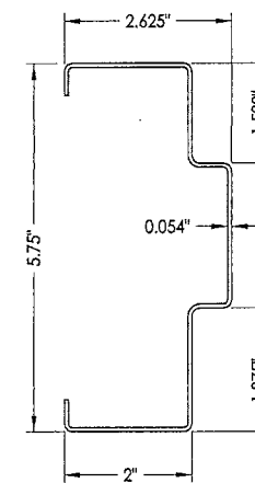
① HOLLOW METAL FRAME
