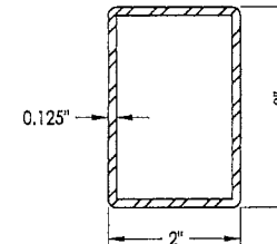
2 MULLION POQ 9200M-11 SERIES
