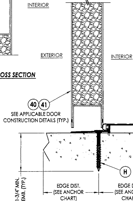
2 6 VERTICAL CROSS SECTION
