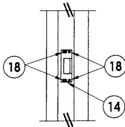
STRIKE DETAIL @ FRAME Rim Panic Exit Device
