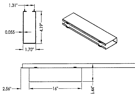
24 CLOSER BOX 16 GA GALV. STEEL
