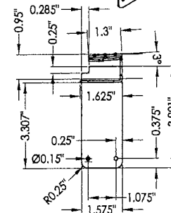
23 CYLINDRICAL LOCK REINFORCEMENT
