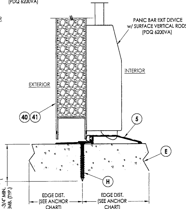
4 6 VERTICAL CROSS SECTION w/ SURFACE VERTICAL RODS
