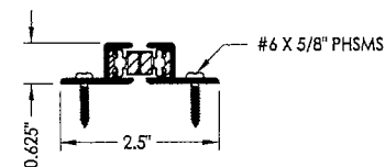
6 ASTRAGAL GASKET
