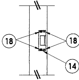
STRIKE DETAIL @ MULLION Rim Panic Exit Device
