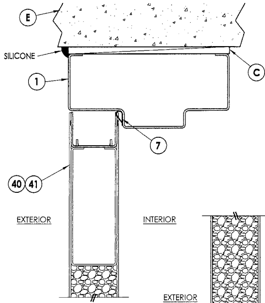
1 6 VERTICAL CROSS SECTION
