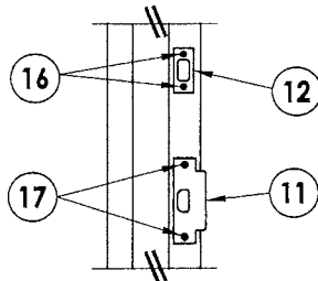
STRIKE DETAIL Latch & Deadbolt
