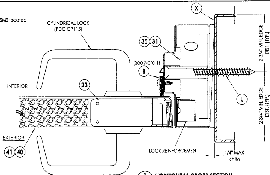
1 4 HORIZONTAL CROSS SECTION CYLINDRICAL LOCK (PDQ)
