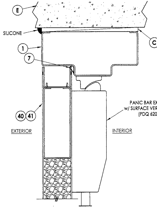
3 6 VERTICAL CROSS SECTION w/ SURFACE VERTICAL RODS
