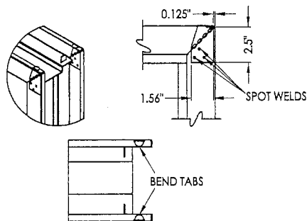
FRAME CORNER DETAILS
