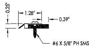
8 FRAME WEATHERSTRIP
