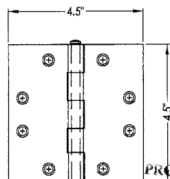
9 STEEL HINGE 0.134" THICK
