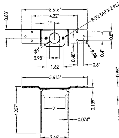
23 CYLINDRICAL LOCK REINFORCEMENT
