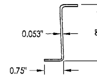
3 "T" ASTRAGAL
