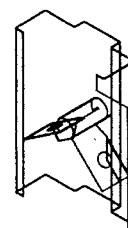
31 EMA BUTTERFLY ANCHOR 18 GA STEEL
