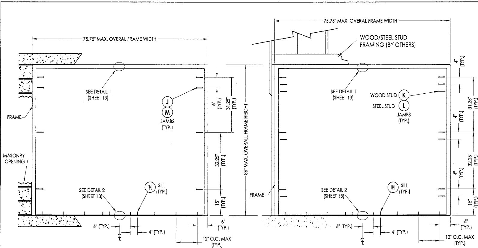
FRAME ANCHORING Masonry Construction Concrete Anchors
