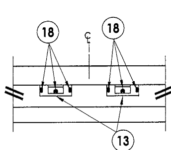
DETAIL 1 Vertical Surface Rod Strike Plate @ Head
