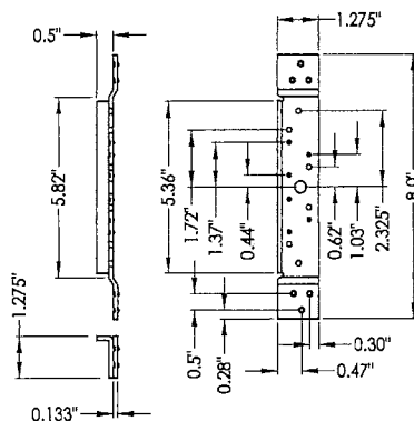
20 HINGE REINFORCEMENT 10 GA STEEL
