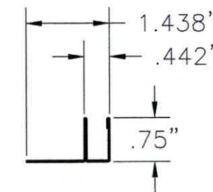
2 F-CHANNEL ALUMINUM 0.022" THICK
