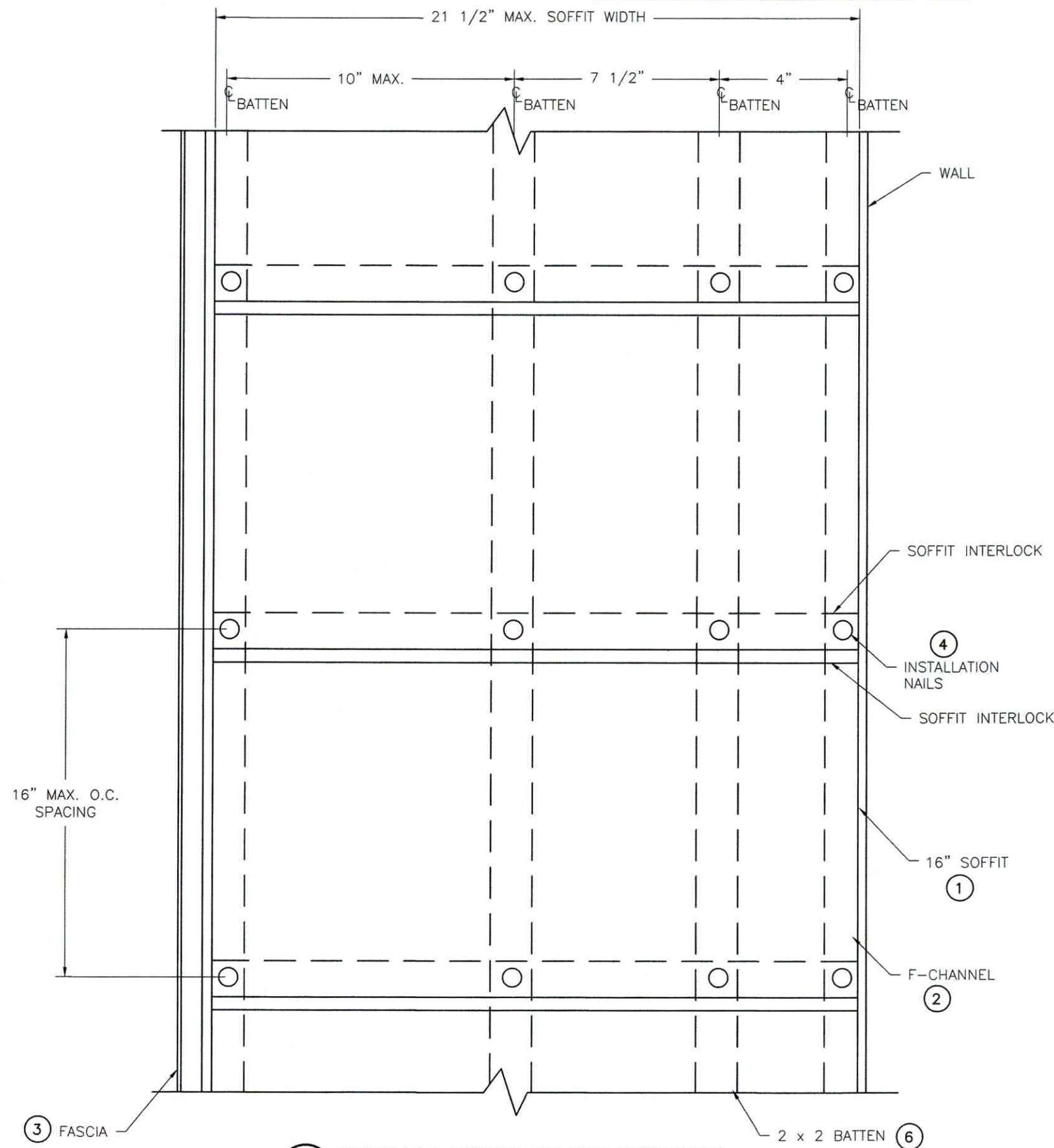
B 4 INSTALLATION CROSS SECTION SP-600 SOFFIT
