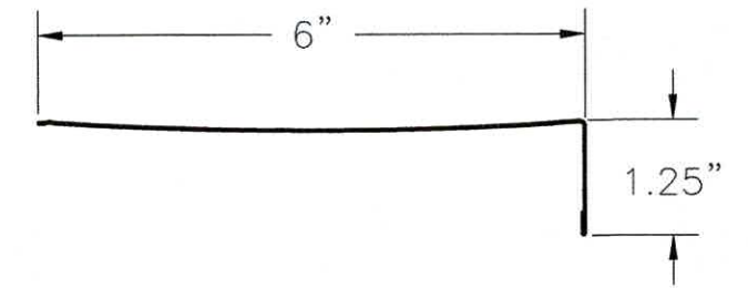
3 6" FASCIA ALUMINUM 0.022" THICK
