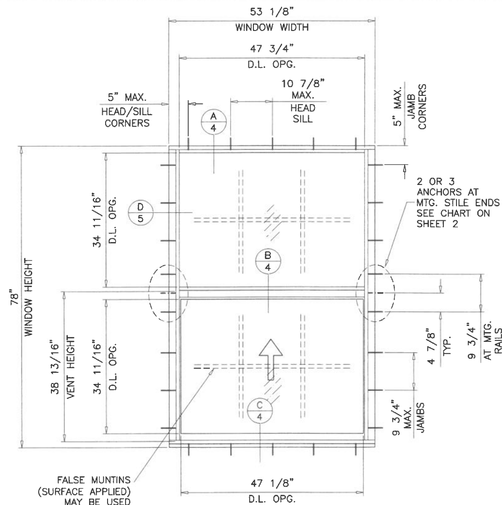
TYPICAL ELEVATIONS
