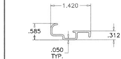
③ SILL TRACK
