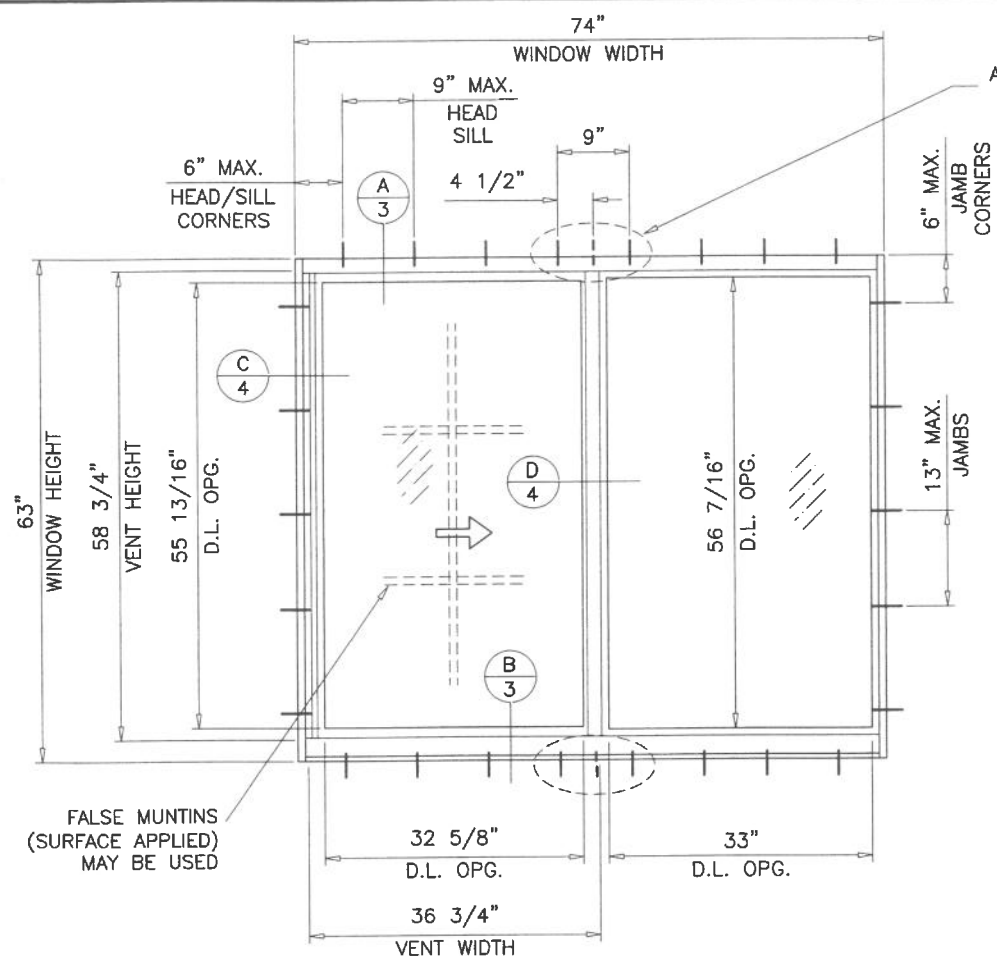
TYPICAL ELEVATIONS
