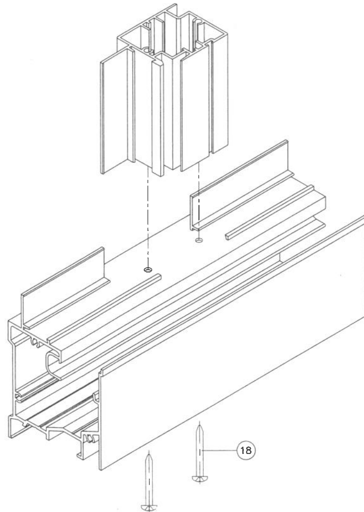
FIXED MTG. RAIL CORNER
