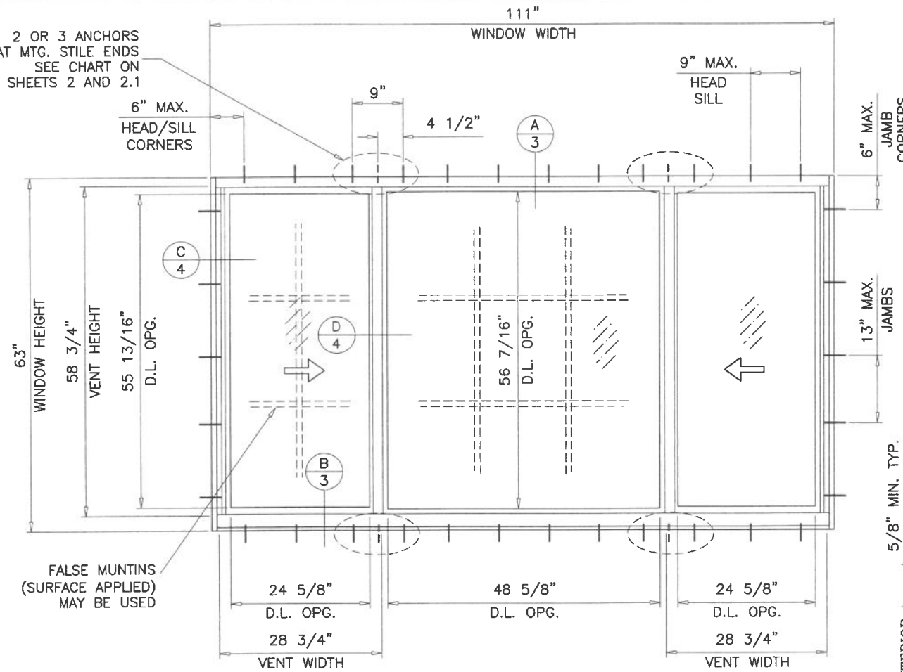
TYPICAL ELEVATIONS
