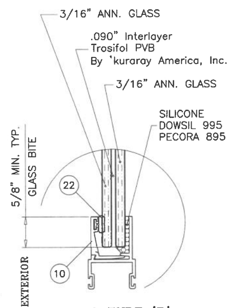
GLASS TYPE 'B'
