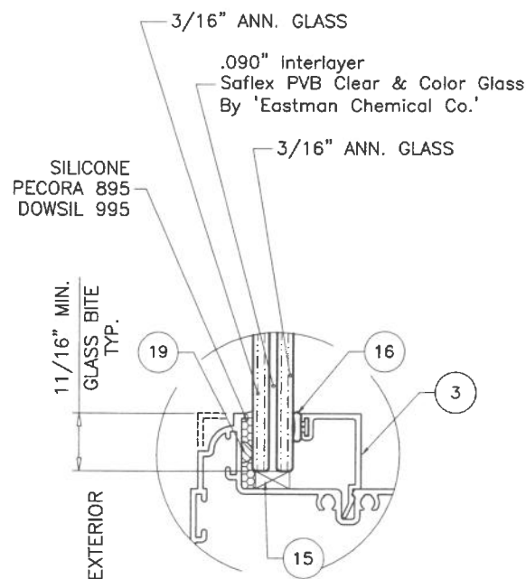
GLASS TYPE 'G2L' 7/16" OVERALL NOM.
