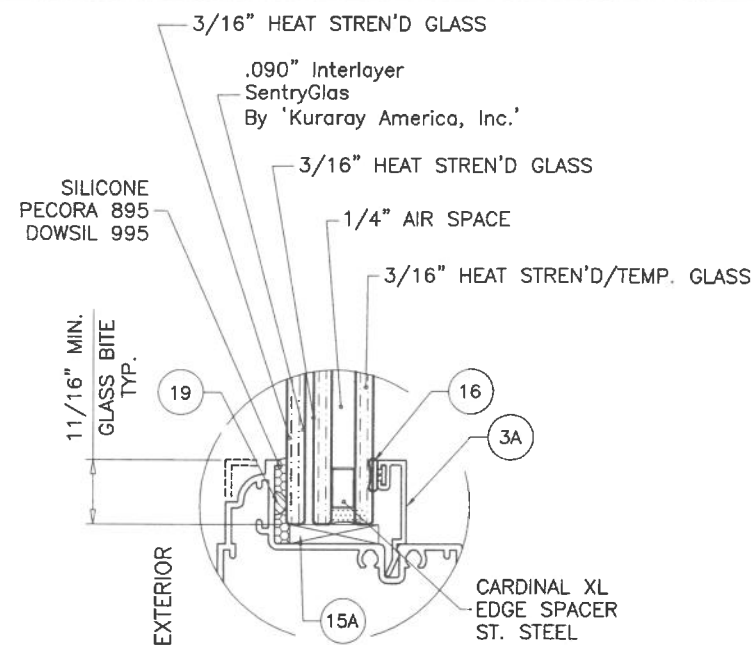
GLASS TYPE 'G1i' 1" OVERALL NOM.
