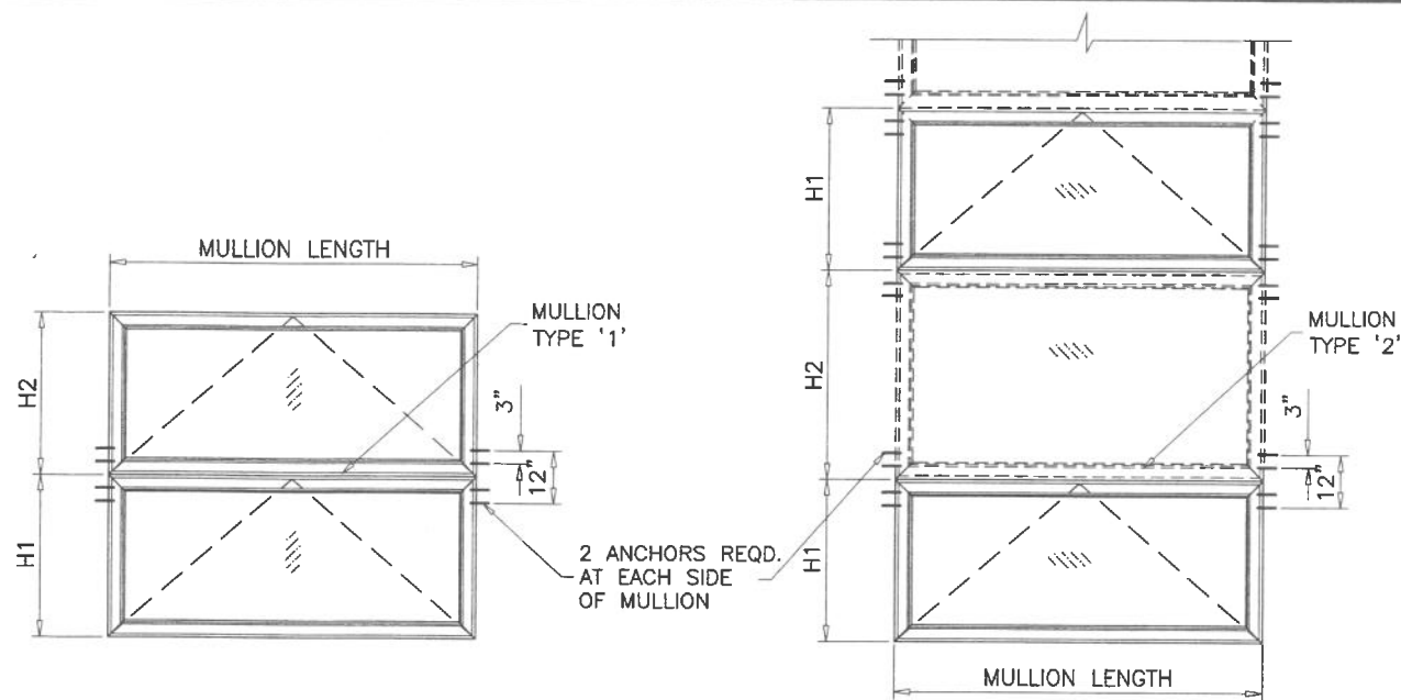
TYPICAL ELEVATIONS SIDE BY SIDE WINDOWS SIDE BY SIDE APPLIES TO TWO OR MORE WINDOWS
