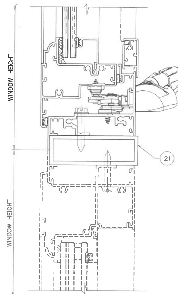
MULLION TYPE '2'
