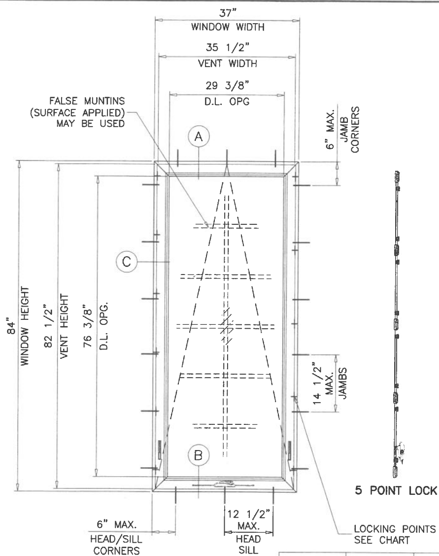
TYPICAL ELEVATIONS TESTED UNITS
