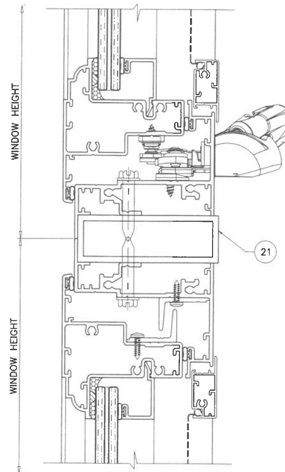
MULLION TYPE '1'
